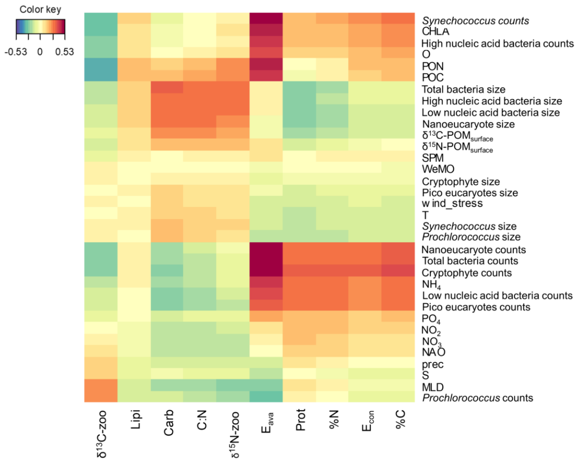
Fig. 7 Clustered image map of the Partial Least Squares analysis performed on environmental (including cytometry data and subsurface isotope ratio of the POM) and zooplankton series from 2010 to 2020.
