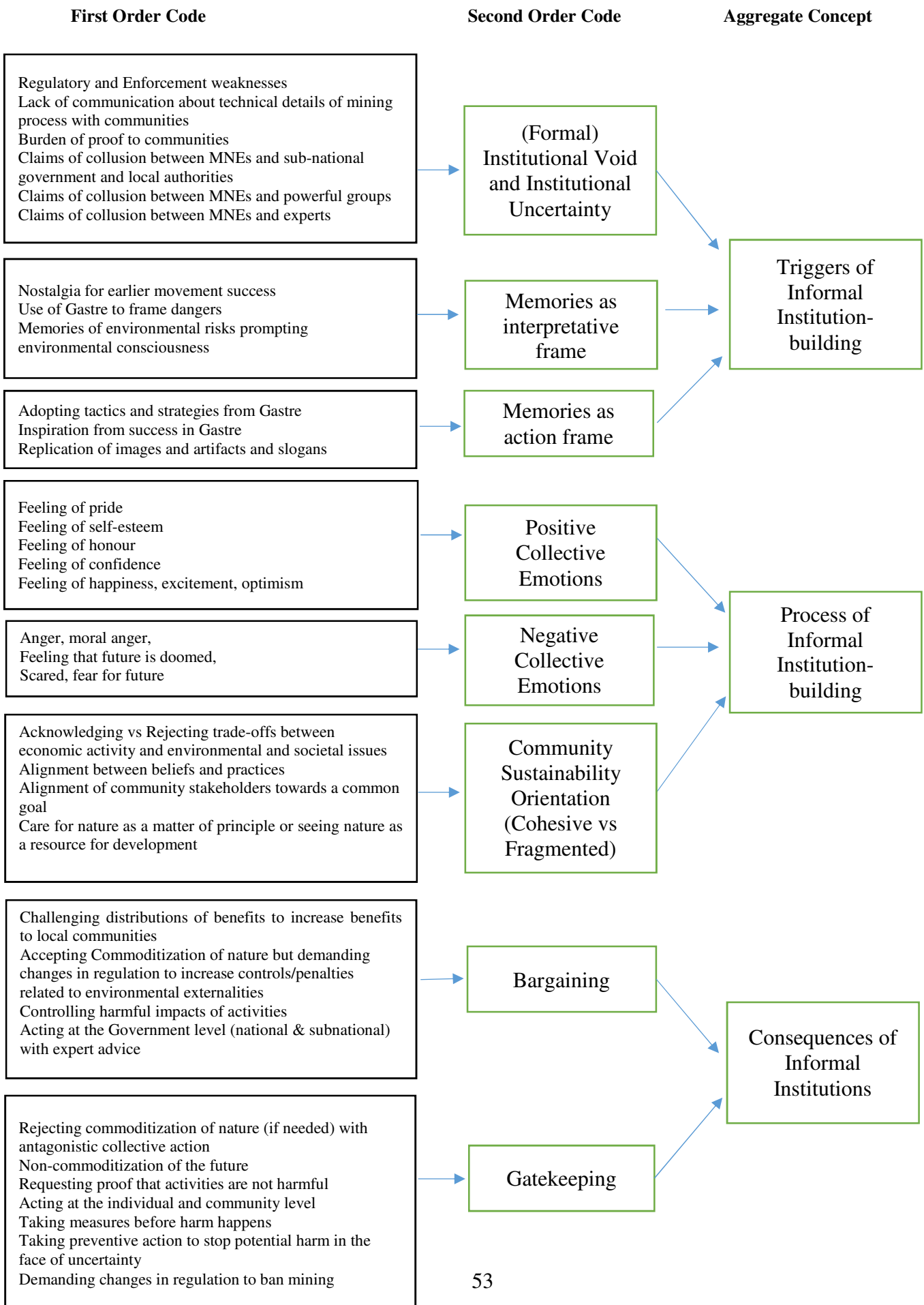
Figure 1: Coding Scheme
