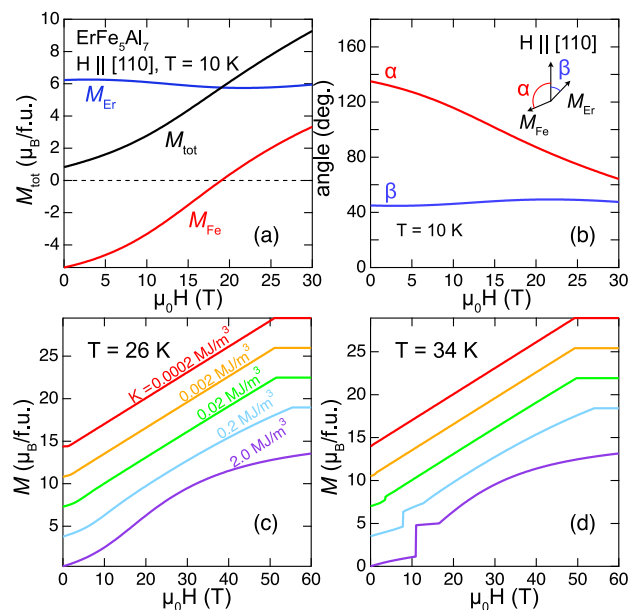
FIG. 6. (a) Field dependence of the Er ( M_{\text{Er}} ), Fe ( M_{\text{Fe}} ), and total magnetization ( M_{\text{tot}} ) at 10 K simulated by the two-sublattice model. (b) Field-dependent angles \alpha and \beta defined with respect to the magnetic field (see inset). M_{\text{tot}} as a function of magnetic fields simulated for the selected anisotropy constants at (c) 26 K and (d) 34 K. The simulated results for different K are vertically shifted for clarity.
