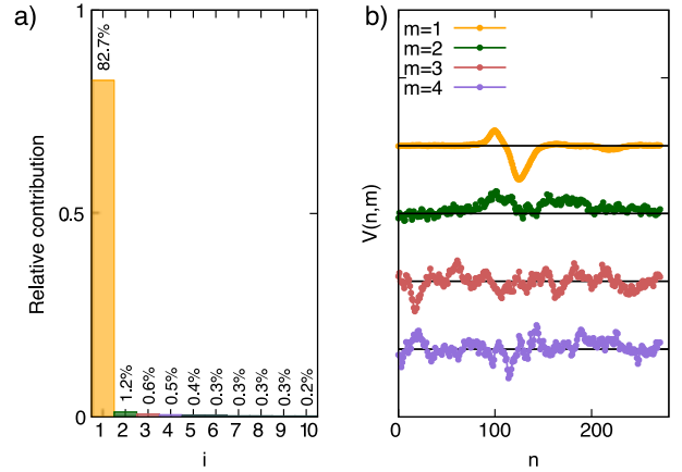
FIG. 9. SVD analysis for the Er L_3 -edge XMCD spectral data. (a) Contribution of components to the variance of the dataset [Fig. 5(b)]. (b) First four components.
