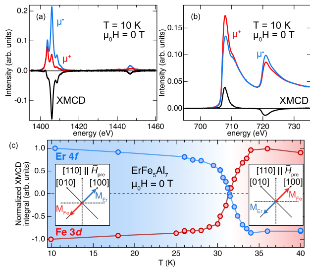
FIG. 2. XAS and XMCD spectra measured using circularly polarized light, \mu^+ and \mu^- , at the (a) Er M and (b) Fe L edges at 10 K under zero magnetic field. (c) Er M_5 - (blue) and Fe L_3 -edge (red) XMCD integrals as function of temperature under zero magnetic field. The signs of the integrals are reversed with respect to (a) and (b). The ferrimagnetic configuration in the red- and blue-colored area is shown schematically in the insets (see text for details). All the XMCD spectra were measured after applying a 30-T magnetic-field pulse along the [110] axis. \vec{H}_{\text{pre}} indicates the direction of the magnetic field pulse.
