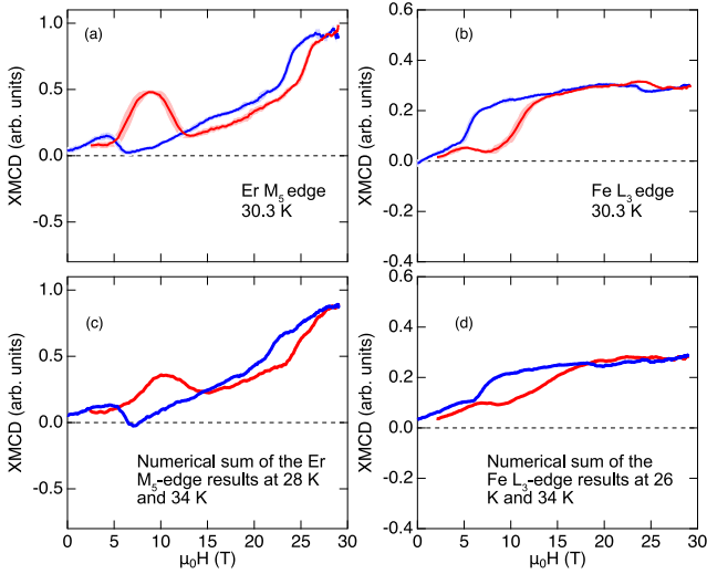
FIG. 8. Field-dependent XMCD amplitude at 30.3 K at the (a) Er M_5 edge and (b) at the Fe L_3 edge. Numerical sum of the field-dependent XMCD amplitudes (c) at the Er M_5 edge at 28 and 34 K and (d) at the Fe L_3 edge at 26 and 34 K. Red and blue lines are data from up and down field sweeps.
