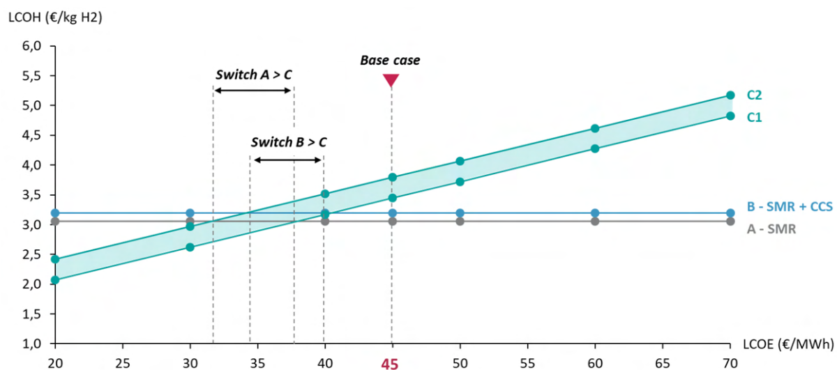
Figure 13 – LCOH sensitivity to electricity supply price (NG price = 40 €/MWh, WACC = 8%, ETS price = 100€/ton of CO 2 , capacity factor = 51%)
