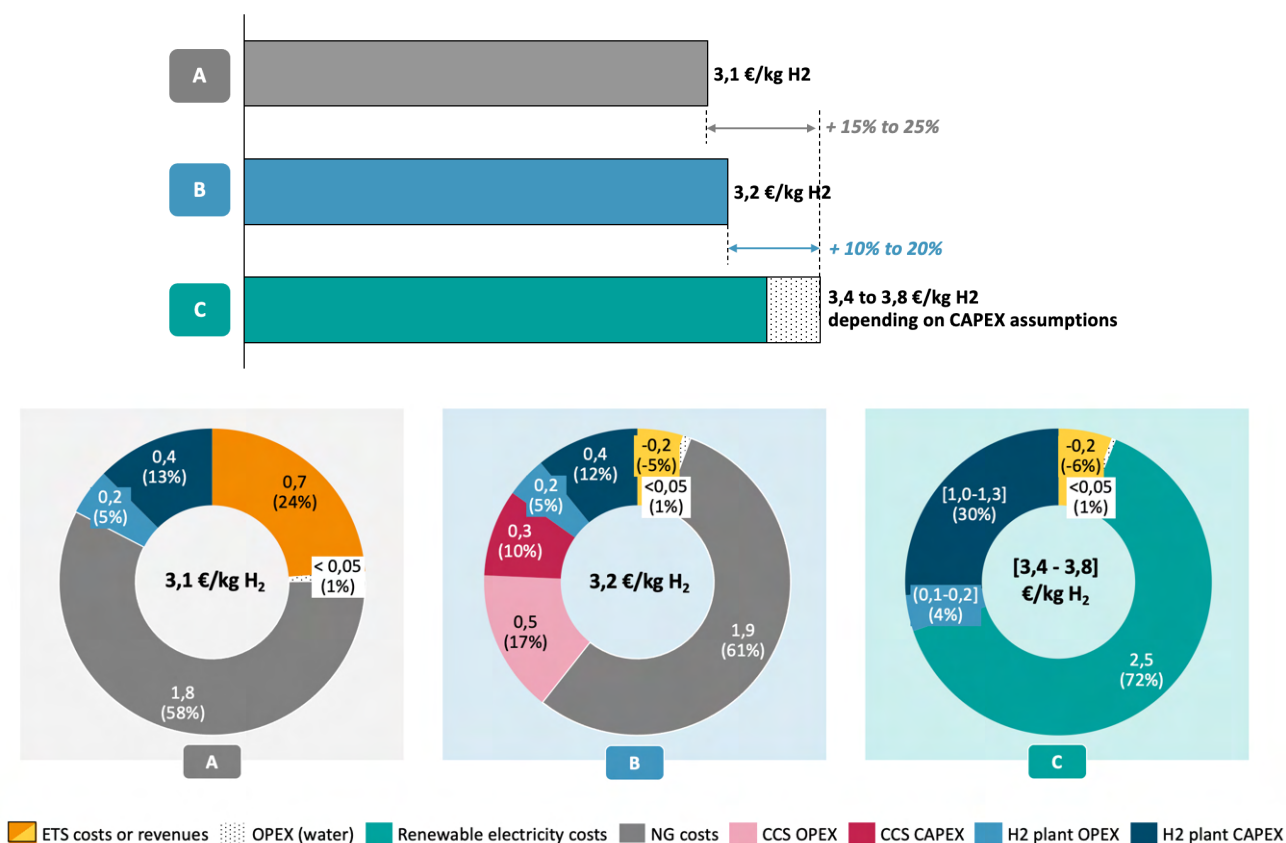
Figure 11 – Base case LCOH in scenario A, B and C (NG price = 40 €/MWh, WACC = 8%, ETS price = 100€/ton of CO 2 , offshore wind LCOE = 45 €/MWh, electrolyser capacity factor = 51%)
