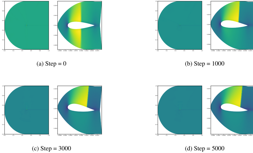
Figure 9: Design optimization of a NACA-Airfoil.
