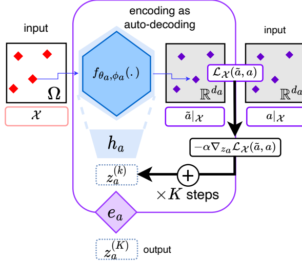
Figure 4: Starting from a code z_a^{(0)} = 0 , the input encoder e_a performs K inner steps of gradient descent over z_a to minimize the reconstruction loss \mathcal{L}_\chi(\tilde{a}, a) and outputs the resulting code z_a^{(K)} of this optimization process. During training, we accumulate the gradients of this encoding phase and back-propagate through the K inner-steps to update the parameters \theta_a and w_a . At inference, we encode new inputs with the same number of steps K and the same learning rate \alpha , unless stated otherwise. The output encoder works in the same way during training, and is not used at inference.
