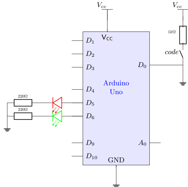
Figure 5: Electric Diagram
