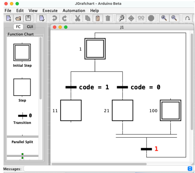
Figure 4: Cash dispenser to JGRAF CET TO ARDUINO
