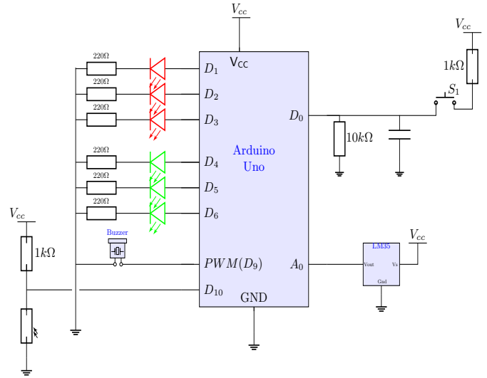
Figure 9: Electric Diagram
