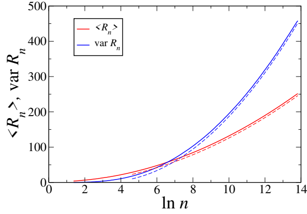
Figure 6. \langle R_n \rangle and \text{Var } R_n plotted against \ln n for uniform points in the unit square. Dashed curves show quadratic fits, slightly offset vertically for greater clarity.
