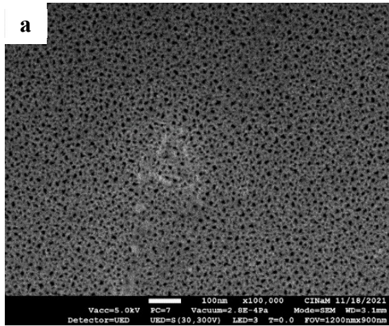
Fig.3 SEM top views (a) and cross sectional views (b) of meso-PS sample
