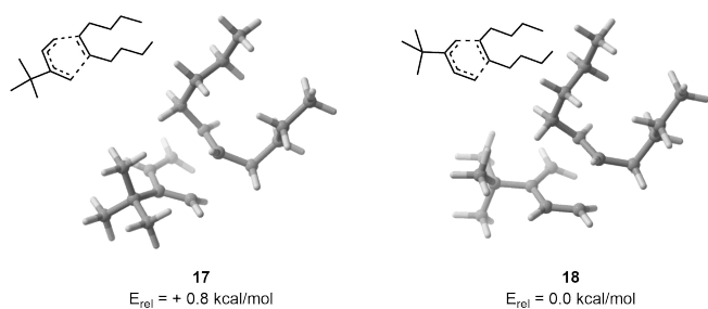
Figure 4 On the left, lowest TS found for endo. On the right, lowest TS found for the exo.
