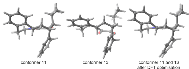
Figure 3 Two conformers found by CREST leading to the same TS after DFT optimisation.
