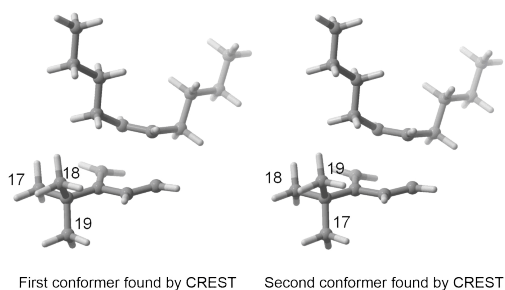
Figure 2 Two conformers found by CREST and considered as duplicates in FASTCAR.
