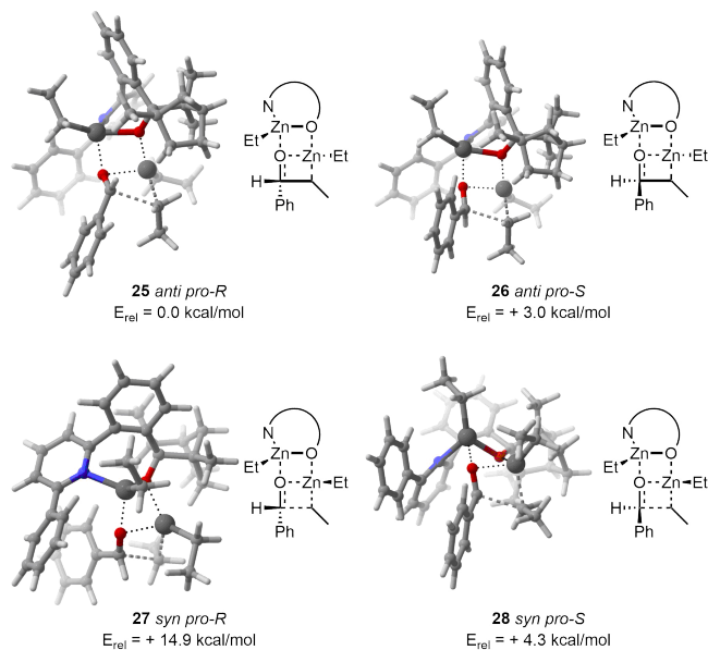
Figure 8 On the top left, lowest TS found for 25 anti pro-R . On the top right, lowest TS found for 26 anti pro-S . On the bottom left, lowest TS found for 27 syn pro-R . On the bottom right, lowest TS found for 28 syn pro-S .
