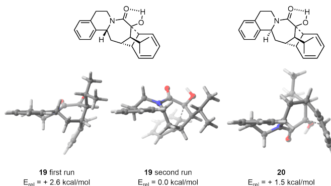
Figure 5 On the left, lowest TS found for major diastereoisomer after the first workflow. On the middle, lowest TS found for major diastereoisomer after a second iteration of the procedure. On the right, lowest TS found for the minor diastereoisomer.
