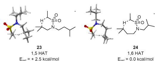
Figure 7 On the left, lowest TS found for 1,5 HAT. On the right, lowest TS found for 1,6 HAT.
