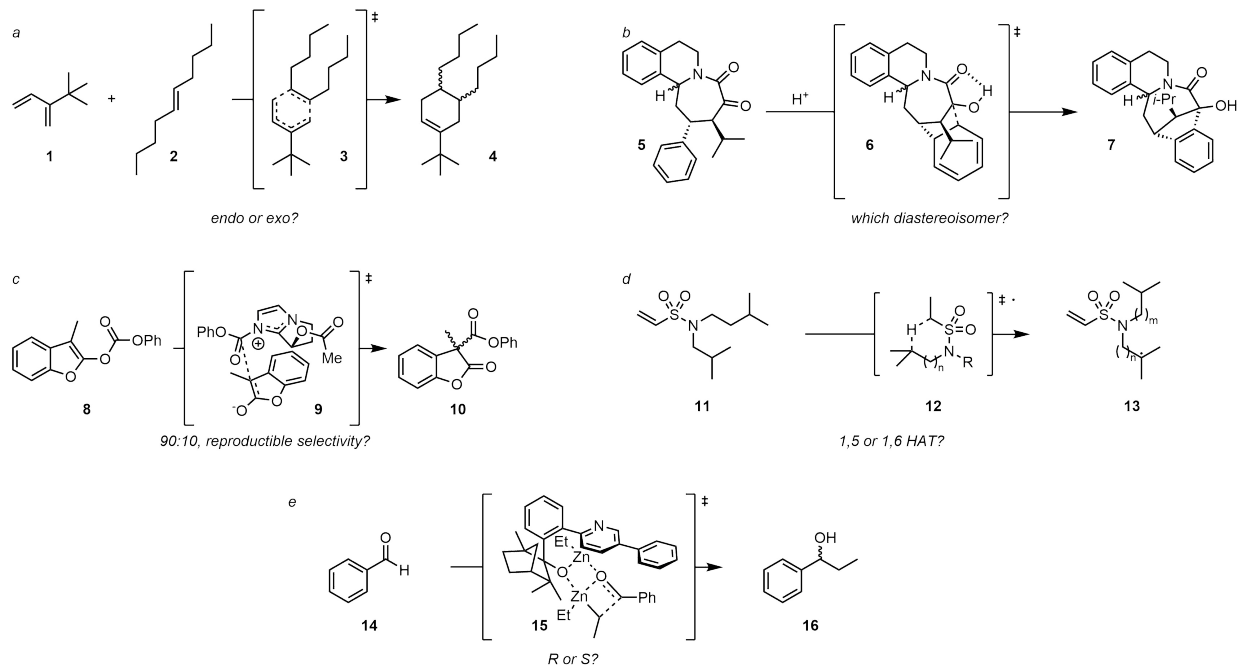
Figure 1 (a) Diels Alder reaction between 4,4-dimethyl-3-methylenepent-1-ene (1) and (E)-dec-5-ene (2). (b) diastereoselective intramolecular acidic cyclization. (c) enantioselective organo-catalysed Black rearrangement. (d) Regioselective intramolecular radical H-atom transfer. (e) Enantioselective dialkylzinc additions on benzaldehyde.
