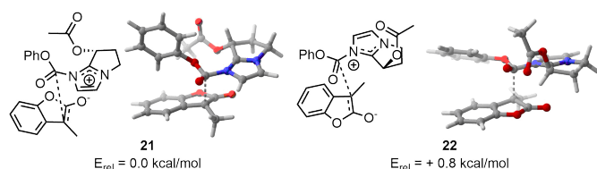
Figure 6 On the left, lowest TS found for major enantiomer. On the right, lowest TS found for the minor enantiomer.
