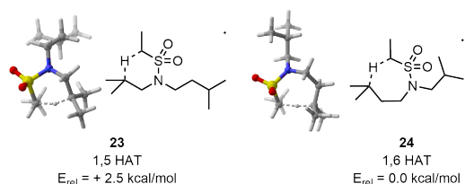
Figure 7 On the left, lowest TS found for 1,5 HAT. On the right, lowest TS found for 1,6 HAT.
