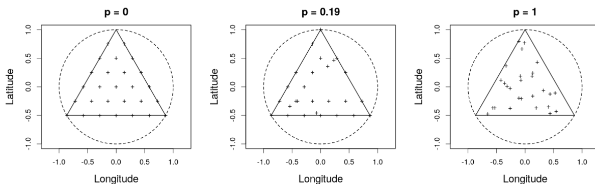
Figure 1 – Effect of the proportion of random sites p on hybrid sampling designs. The triangle is the area of study. Crosses show the position of the 27 sampling points. The middle panel corresponds to p = 5/27 \approx 0.19 .
