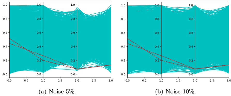
Figure 6: PC plot of the predicted (cyan) and two sets (red) of the ground-truth input parameter values for the observed output variable y that include noise levels: (a) 5% (b) 10%. Datasets are scaled.
