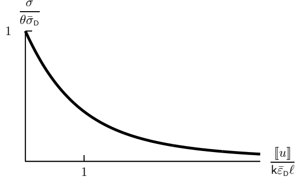
Figure 8: Graph of the cohesive law obtained for n = 1 which gives \sigma in term of [[u]] . Note that the curve is monotonically decreasing, but tends only asymptotically to 0.
