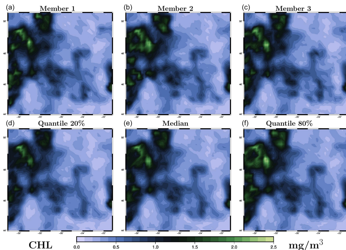
Figure 6. Ensemble analysis obtained with the MCMC sampler for surface chlorophyll concentration (in \text{mg m}^{-3} ) on 26 May 2009. The figure displays three members of the ensemble (a–c) and three quantiles (20 %, 50 % and 80 %) of the marginal ensemble distributions (d–f). The x axis and y axis represent longitude and latitude, respectively.
