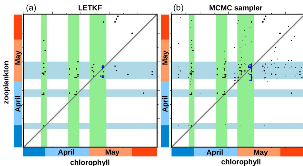
Figure 10. Scatter plot of phenology (in days) for chlorophyll ( x axis) and zooplankton ( y axis). At 47.25° N, 26° W. With the LETKF algorithm (a) and the MCMC sampler (b). Prior ensemble (black), augmented prior (small black dots), and analysis (blue).
