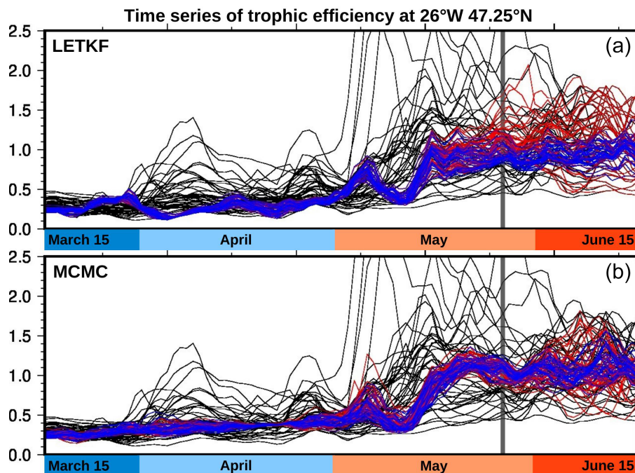
Figure 12. Time series of trophic efficiency. At 47.25^{\circ} N, 26^{\circ} W. With the LETKF algorithm (a) and the MCMC sampler (b). Prior (black), analysis (blue), and forecast (red).
