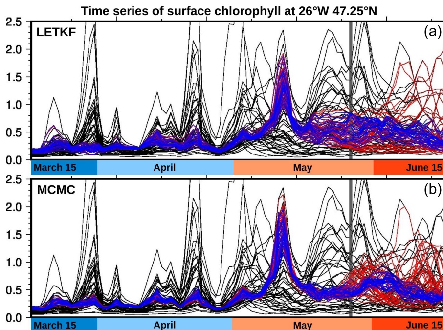
Figure 4. Ensemble surface chlorophyll time series at 47.25^{\circ} N, 26^{\circ} W. The black curves represent 40 members of the prior ensemble (as produced by the NEMO–PISCES simulator), the blue curves represent 40 members of the ensemble analysis (using observations for the entire period), and the red curves represent 40 members of the ensemble forecast (using only observations until 25 May). The forecast thus starts on 25 May (vertical grey line). These results are shown for the LETKF algorithm (a) and the MCMC sampler (b).
