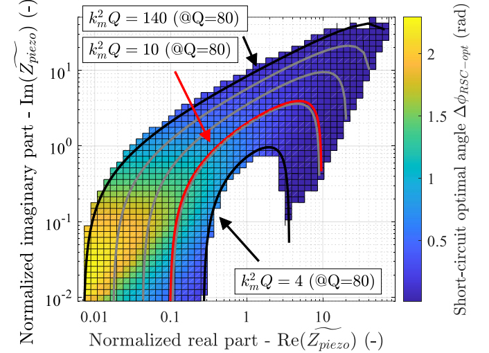
Fig. 6. 50x50 map of short-circuit angle versus normalized impedance \widetilde{Z}_{piezo} . Lines for specific values of k_m^2 Q are drawn on top of the map. Background color is equivalent to \Delta\phi_{RSC-opt} = 0 rad. Characteristics of our harvester, presented in section V, are shown in red.
