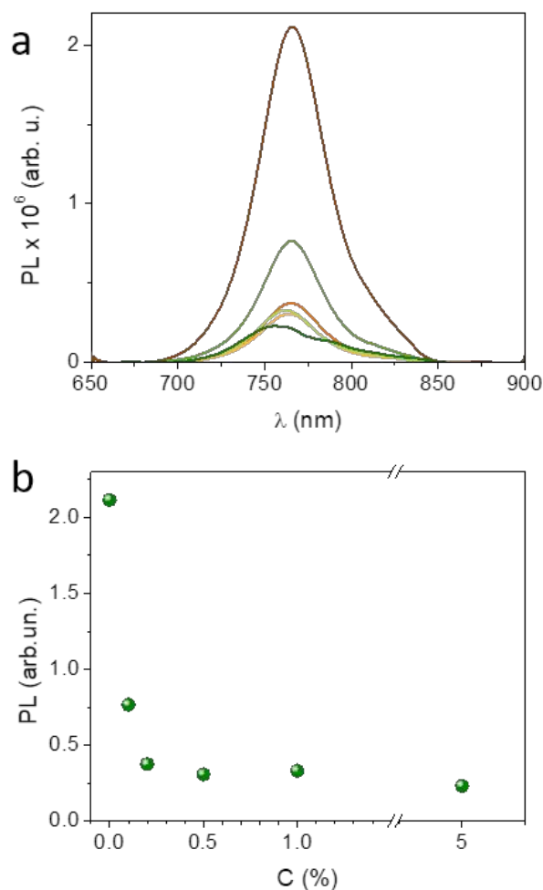
Fig. 4. Photoluminescence as a function of the doping concentration.
