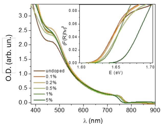
Fig. 2. UV-vis absorption spectra and Tauc plots in the inset.
