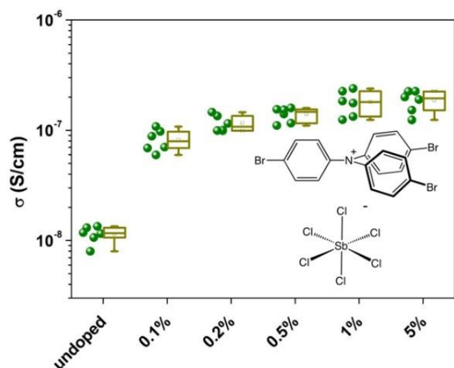
Fig. 1. Conductivity as a function of doping concentration.
