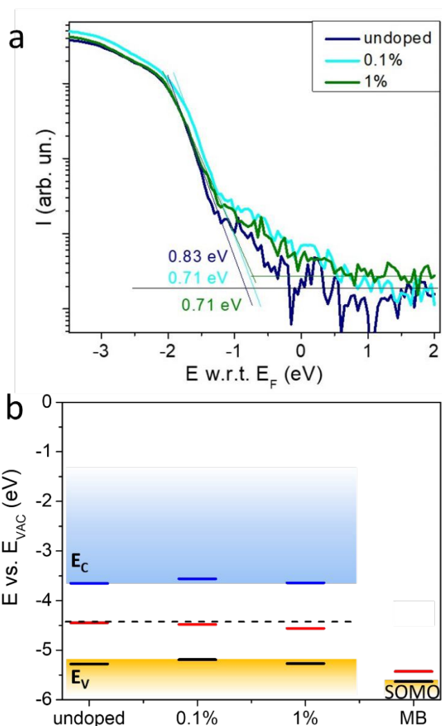
Fig. 5. a) Valence band region of the UPS spectra for undoped and doped MAPI. b) E_F shift upon doping with MB as well as the SOMO and E_F of a MB thin film. The SOMO level of MB is estimated from UPS assuming that it is the highest (partly) occupied molecular orbital. E_c and E_v represent the energy of the conduction and valence band of MAPI, respectively. Filled states are black, empty blue, and E_F red.
