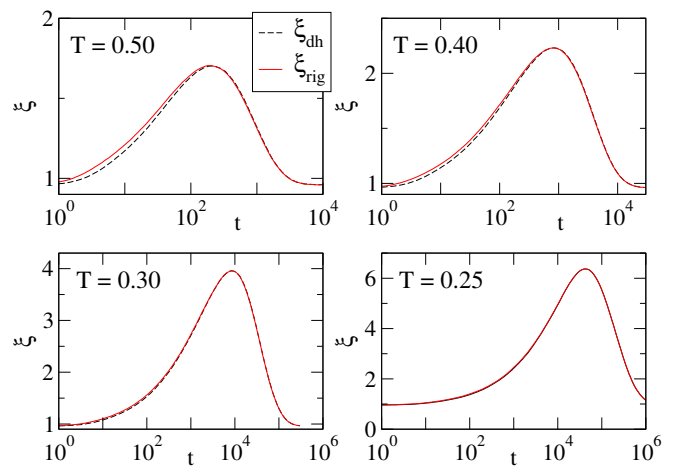
FIG. 6. Dynamic lengths \xi_{\text{dh}} (dashed line) and \xi_{\text{rig}} (full line) as a function of time t in the kinetically constrained spin model, for different values of temperature T . Parameters: K = 1 , N = 10^3 .
