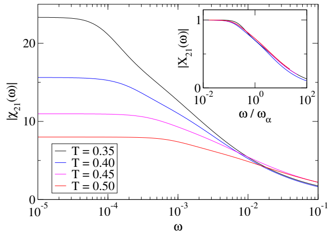
FIG. 4. Modulus |\chi_{21}(\omega)| of the third-order response for different values of temperature ( T = 0.35, 0.40, 0.45, 0.50 , from top to bottom) in the kinetically constrained spin model. No peak is observed, and |\chi_{21}(\omega)| decreases monotonically with frequency. Inset: corresponding rescaled response |X_{21}(\omega)| versus rescaled frequency \omega/\omega_\alpha(T) . Parameters: K = 1 , N = 10^3 . The third-order response is obtained from C(t, E_0) - C(t, 0) evaluated for E_0 = 0.13, 0.15, 0.18, 0.20 at temperature T = 0.35, 0.40, 0.45, 0.50 , respectively.
