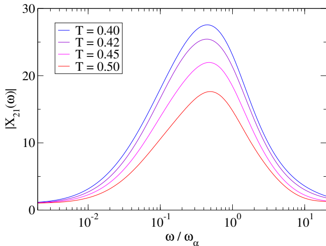
FIG. 3. Modulus |X_{21}(\omega)| of the rescaled third-order response in the spin model with stochastic couplings, as a function of the rescaled frequency \omega/\omega_\alpha(T) , for different values of temperature ( T = 0.40, 0.42, 0.45, 0.50 , from top to bottom; same data as Fig. 2). The peak value increases when decreasing temperature.
