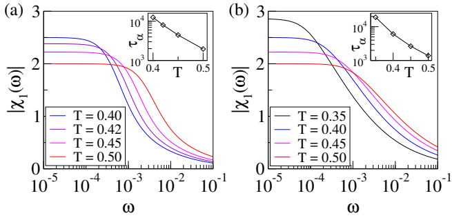
FIG. 1. Modulus of the linear response \chi_1(\omega) as a function of the angular frequency \omega , for different values of temperature (same color code on both panels). (a) Spin model with stochastic couplings for T = 0.40, 0.42, 0.45, 0.50 , from top to bottom at low \omega ( J_0 = 1, B = 3 ). Inset: relaxation time \tau_\alpha = 2\pi/\omega_\alpha vs. temperature T , where \omega_\alpha is the angular frequency at which the imaginary part \chi_1''(\omega) is maximum. (b) Kinetically constrained spin model for T = 0.35, 0.40, 0.45, 0.50 , from top to bottom at low \omega ( K = 1 ). Inset: \tau_\alpha vs. T . In both cases, the response function decays monotonously with frequency. System size: N = 10^3 for (a) and (b).
