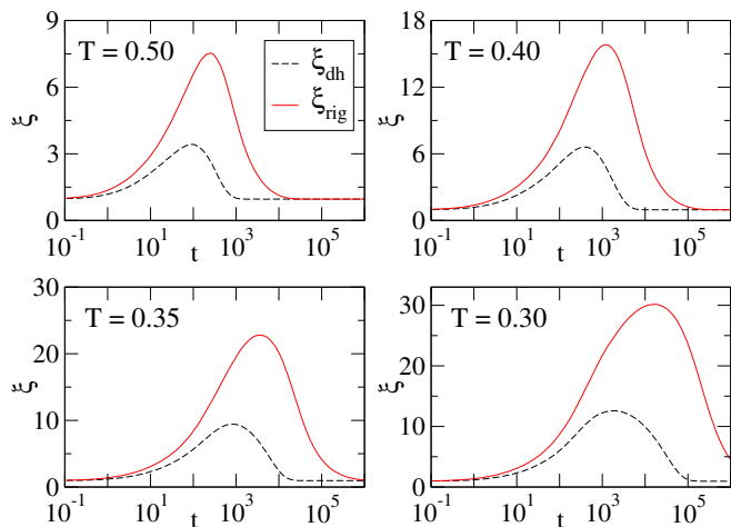
FIG. 5. Dynamic lengths \xi_{\text{dh}} characterizing dynamical heterogeneities (dashed line) and \xi_{\text{rig}} characterizing cooperative effects (full line) as a function of time t in the spin model with stochastic couplings, for different values of temperature T . Note that the Y -axis scale changes from one panel to the other to enhance readability. At low temperature, \xi_{\text{rig}}(t) becomes much larger than \xi_{\text{dh}}(t) for t \gtrsim \tau_\alpha , showing that interactions play the role of a restoring force -see VIA 2- when couplings change very slowly. Parameters: J_0 = 1 , B = 3 , N = 10^3 .
