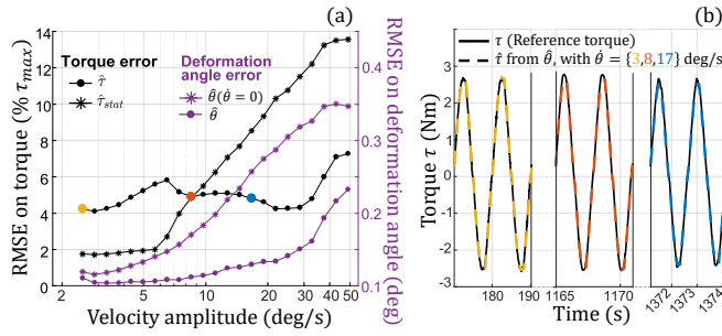
Fig. 7. Torque estimator assessment. (a) Root Mean Square Error (RMSE) on \tau and \theta with different estimators, considering or not the dynamic part of the torque estimate ( \hat{\tau} and \hat{\tau}_{stat} respectively). Deformation angles ( \hat{\theta} ) are estimated considering or not the effect of velocity change. (b) Torque estimator temporal behavior at three different velocities, emphasized with colored dots on the left plot.
