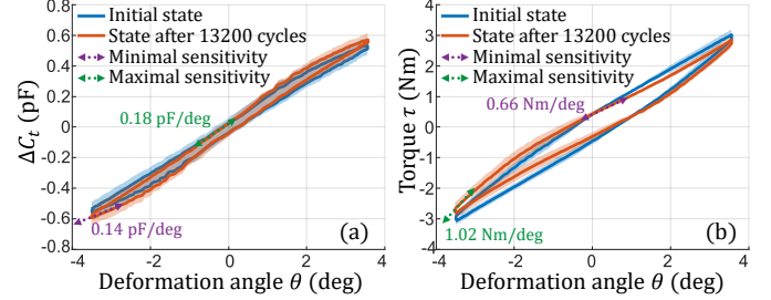
Fig. 6. Durability and repeatability results. Plots show the mean \pm standard deviation of capacitance (a) and torque (b) characteristics between the five printed sensors initially and after the durability trial. Extreme sensitivities within the measurement range are also indicated.
