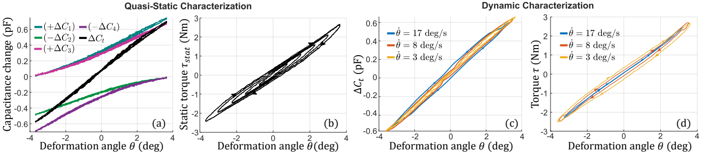
Fig. 4. Torque sensor characterization. Relationship between deformation angle and capacitance change (a) or torque (b) in quasi-static conditions for different angle amplitudes. (c) and (d) show the dependence of these relationships with the angular deformation velocity \dot{\theta} .
