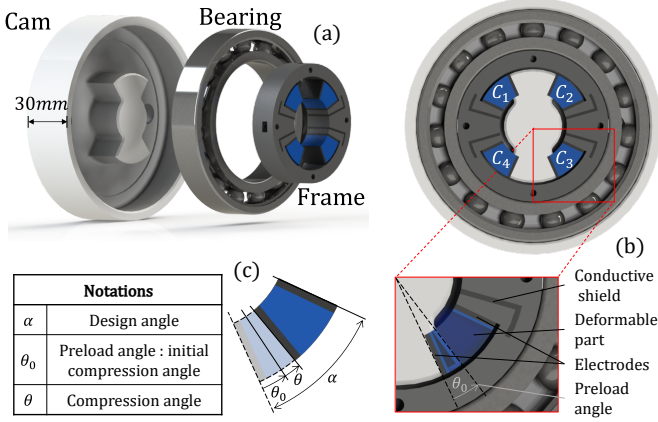
Fig. 2. Design of the proposed torque sensor. (a) General view showing the sensor parts. (b) Capacitive structure components. (c) Notations for the capacitive structures.
