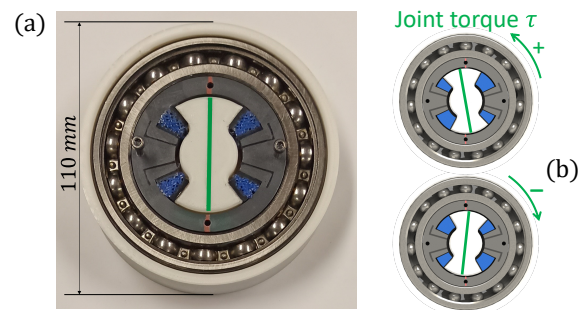
Fig. 1. (a) Picture of the proposed torque sensor. (b) Behavior under torque: for a given torque direction, two deformable capacitive structures are compressed while the other ones are relaxed.
