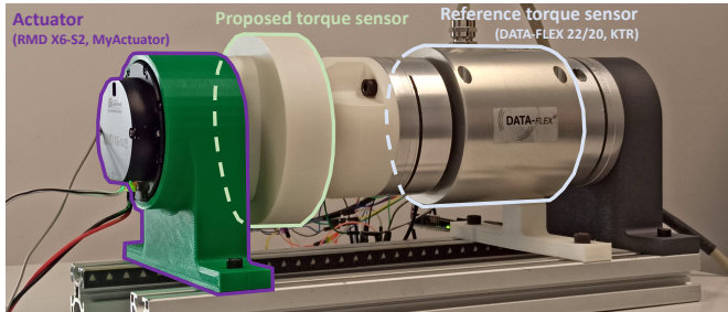
Fig. 5. Experimental setup. A BLDC motor actuates the proposed torque sensor while measuring the deformation angle \theta . An external torque sensor measures the reference torque \tau .
