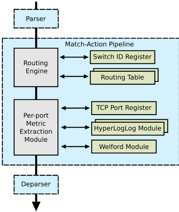
Fig. 3. P4 architecture.
