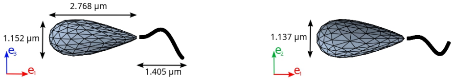
FIG. 16. Optimal monoflagellated swimmer ( water-drop swimmer ) obtained by optimizing all parameters describing the head and flagellum, taking into account the mean velocity problem J_1 (13) in the frame (e_1, e_3) (Left) and in the frame (e_1, e_2) (Right).
