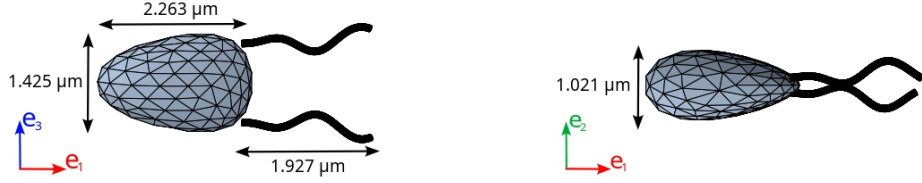
FIG. 19. Optimal biflagellate swimmer obtained by optimizing all parameters describing the head and flagellum, taking into account the mean efficiency problem J_2 (13) in the frame (e_1, e_3) (Left) and in the frame (e_1, e_2) (Right).
