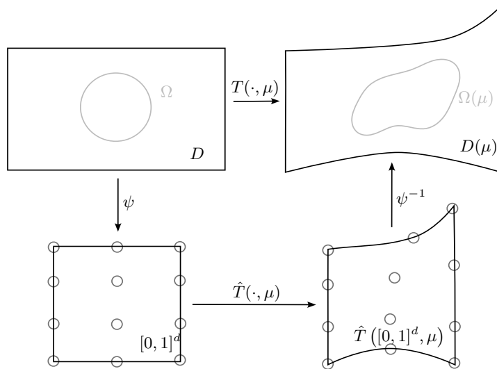
FIG. 3. Illustration of the FFD method deforming a domain D containing a \Omega shape via a \mu vector using the T application described by (9).
