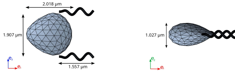
FIG. 14. Optimal swimmer obtained by the head optimization of the literature swimmer from [10] in the frame (e_1, e_3) (Left) and in the frame (e_1, e_2) (Right).
