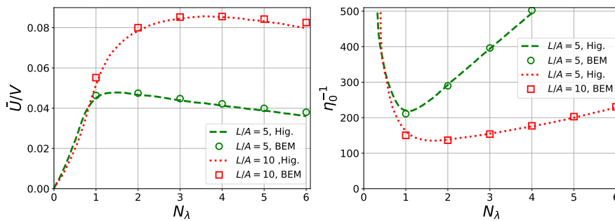
FIG. 11. Comparison of normalized mean translational velocity (Left) and the inverse efficiency (Right) between the results obtained in [9] (dashes) and our simulations for L/A = 5 (round) and L/A = 10 (square).
