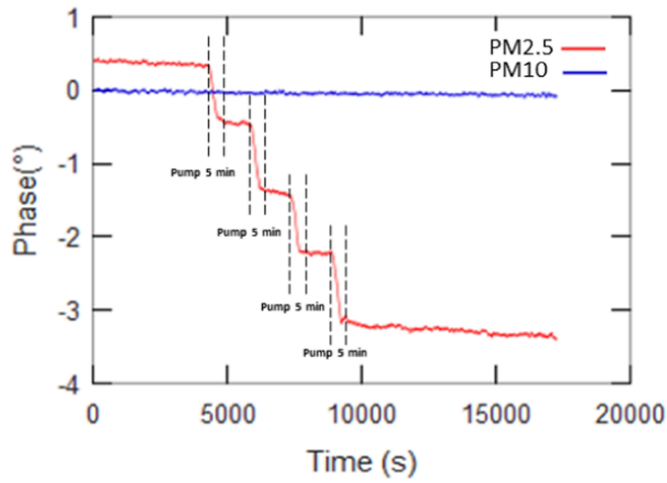
Fig. 11. SAW sensor phase shift of PM2.5 stage (red) and PM10* (blue) during successive exposures to particles in the [0, 2.5 μm] range.
