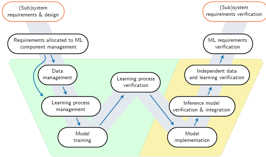
Figure 3: The learning phase (in green) and the inference phase (in yellow) in the W development process of an assured ML solution (EASA, 2020; EASA, 2021b)
