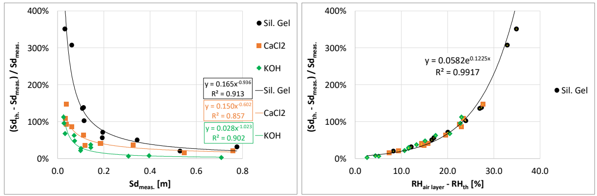
Figure 7: Relative differences between Sd_{meas.} and Sd_{th} as function of Sd_{meas.} (a) and of RH_{air\ layer} - RH_{th} (b) with the three desiccants and for all materials.
