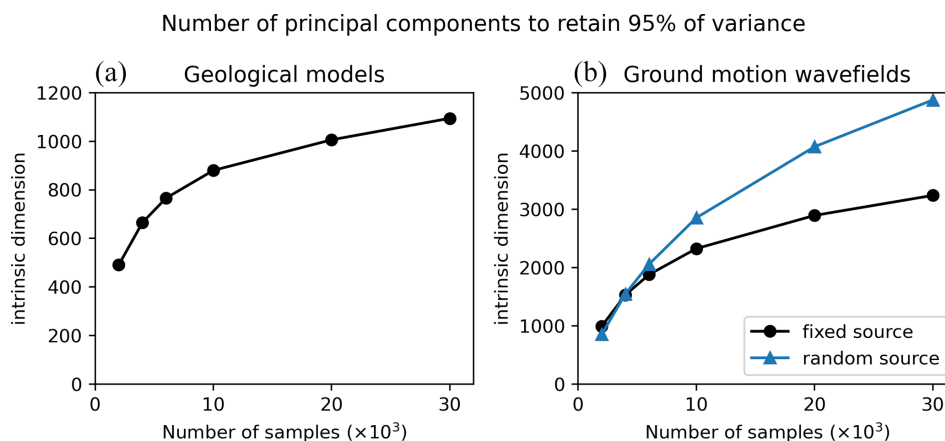
Figure B1. Number of principal components (y axis) required to represent 95 % of the variance in data as a function of the dataset size (x axis) for geological models (a) and ground motion wavefields (b). For ground motion, the HEMEW-3D database is used for the fixed source (black line) and the HEMEW S -3D database corresponds to the blue line.
