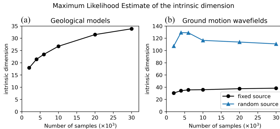
Figure B4. Intrinsic dimension estimated by the MLE (y axis) as a function of the dataset size (x axis) for geological models (a) and ground motion wavefields (b) . For ground motion, the HEMEW-3D database is used for the fixed source (black line) and the HEMEW S -3D database corresponds to the blue line.
