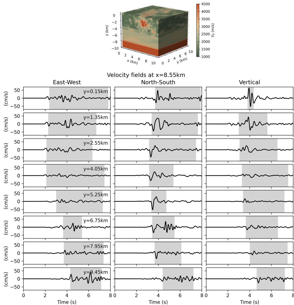
Figure 2. Three-component velocity waveforms synthesized at eight virtual sensors on a line parallel to the y axis at x = 8.85 km. The shaded area extends from 5 % to 95 % of the Arias intensity; hence, its length equals the relative significant duration (RSD). The corresponding geological model is shown at the top. The source is located at (2.04, 3.64, -2.17 ) km. The associated frequency spectra are given in Fig. A3.
