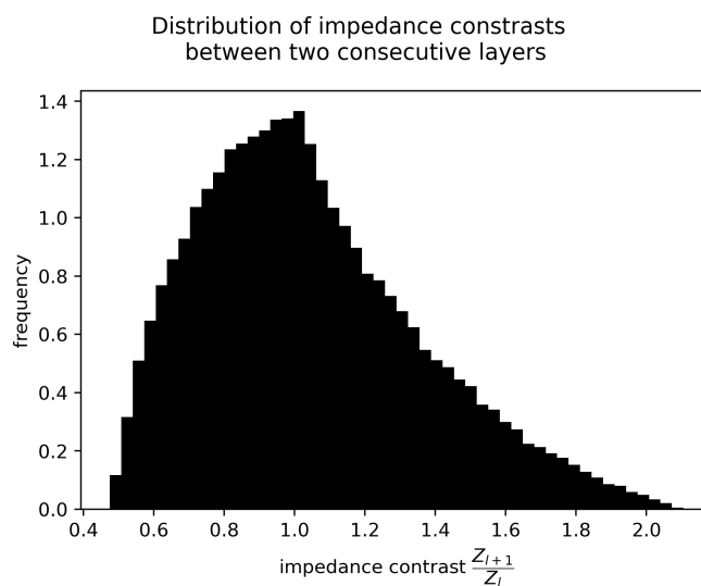
Figure A2. Distribution of impedance contrasts in the HEMEW S -3D database. The impedance contrast is computed as the ratio between impedance in one layer ( Z_\ell = V_{s\ell} \times \rho_\ell ) and impedance in the layer above it ( Z_{\ell-1} ).
