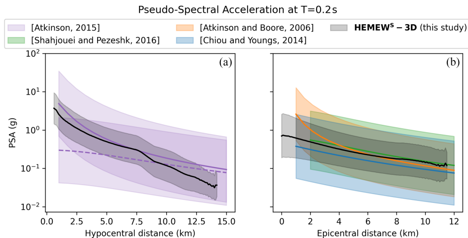
Figure 8. Horizontal PSA at period T = 0.2 s as a function of hypocentral distance (a) and epicentral distance (b) for GMMs by Atkinson (2015), with a depth of 1 km (solid purple line, a); Atkinson (2015), with a depth of 7.5 km (dashed purple line, a); Atkinson and Boore (2006) (orange, b); Chiou and Youngs (2014) (blue, b); Shahjoui and Pezeshk (2016) (green, b); and our HEMEW S -3D database (black). Solid lines correspond to the mean PSA and shaded areas to 1 standard deviation. Horizontal PSA is computed as the geometrical mean of east–west and north–south components.
