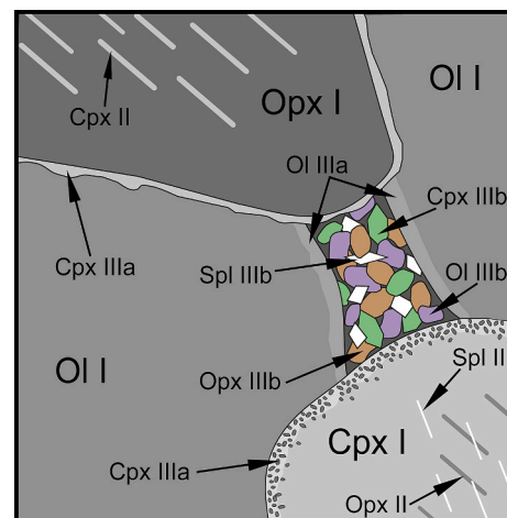
Fig. 2. Sketch illustrating the classification of minerals according to their textural position in mantle peridotite. I – primary mineral grains; II – lamellae in pyroxenes; IIIa – minerals forming reaction rims around primary grains; IIIb – minerals forming fine-grained interstitial aggregates. Modified after Puziewicz et al. (2023) and Tedonkenfack et al. (2021).
