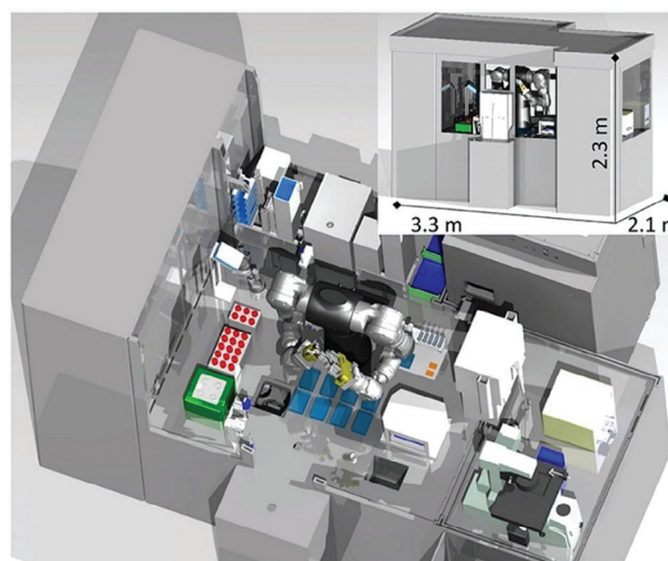
Figure 5. Robotic cell for tissue engineering utilizing a two-arm robot and conventional lab equipment. (Reproduced under the terms of the CC-BY license. [43] Copyright 2021, Haeusner et al.).
