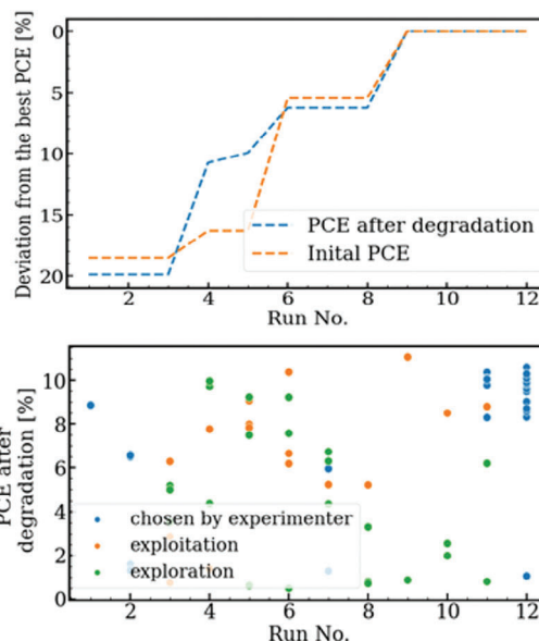
Figure 7. Example of an autonomous optimization of a quaternary OPV-mixture performed on AMANDA/Line1. The Bayesian optimizer Phoenics was used to optimize two objectives (initial efficiency and efficiency after aging test) in a 3D-process parameter space. Six samples were investigated in each iteration, the optimum was found after nine iterations. (Reproduced with permission. [53] Copyright 2021, Tobias Osterrieder.)
