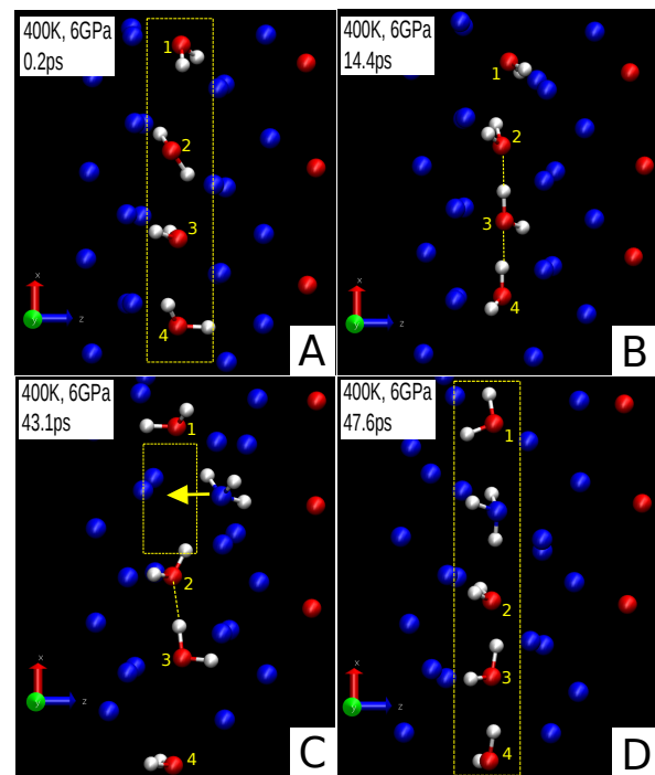
FIG. 5. Snapshots of simulation at 400 K and 6 GPa (see text). Blue, red and white balls are nitrogen, oxygen and hydrogen atoms, respectively. For clarity sake, we did not draw hydrogen atoms that are not directly involved in hydrogen bonds with the diffusing molecules.
