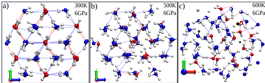
FIG. 2. Snapshots of the simulated AHH alloys at three different temperatures (300, 500 and 600 K) and 6 GPa. The portions of the structures are seen along the a crystal axis of the simulation box, that is, on few (100) planes.
