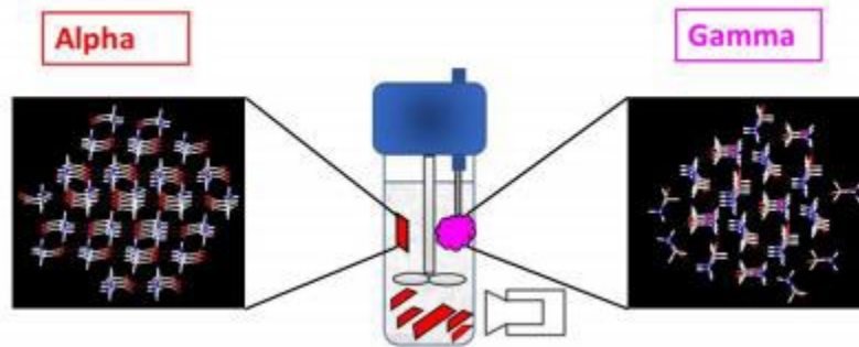
Figure 1: Effect of fluid shear on the polymorphism of a single gamma glycine seed
