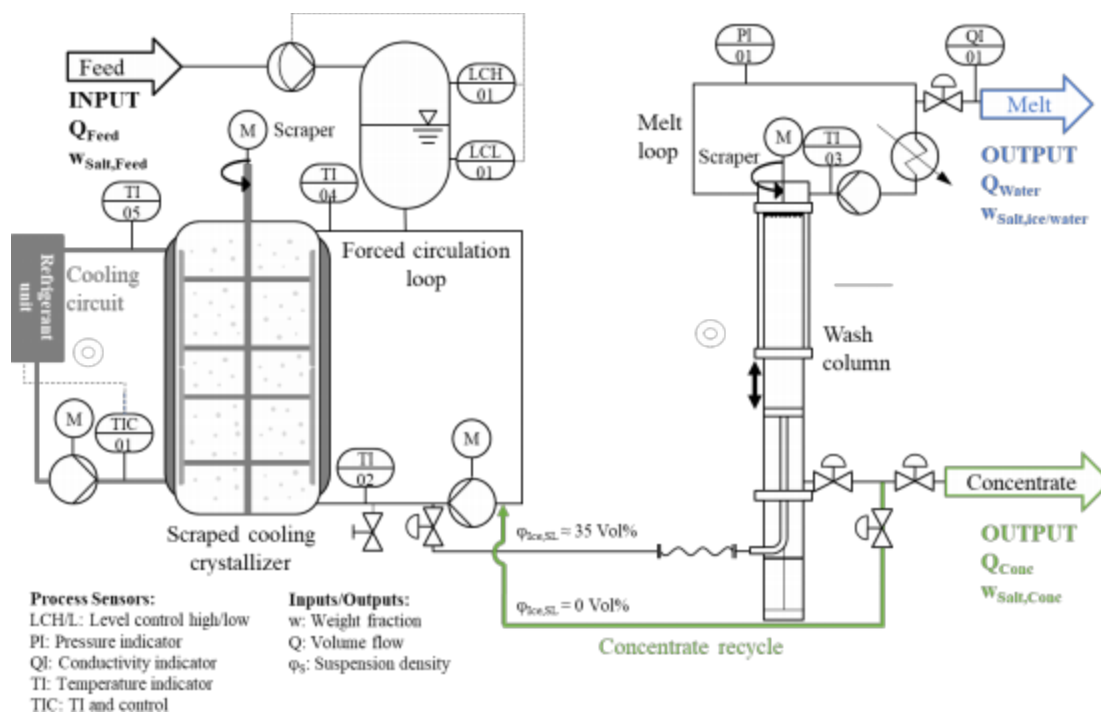
Figure 1: Schematic illustration of the freeze concentration plant (designed by the SULZER CHEMTECH AG) containing the crystallization unit consisting of the scraped cooling crystallizer with a forced circulation loop, the solid-liquid separation unit consisting of a mechanical piston-type wash column with melt loop, and the recycle stream for the concentrate.
