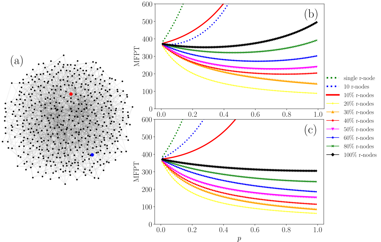
Figure 1: (a) Random search dynamics with resets on a realization of the Barabási-Albert random graphs with N = 500 nodes and attachment parameter m = 4 . Frames (b,c) show the MFPT \langle T_{ij} \rangle of Eq. (43) as a function of the Bernoulli probability p for different relocation scenarios of the searcher. The sets of r-nodes to which resetting is allowed are randomly selected by an independent Bernoulli trial for each node, generating homogeneously distributed fractions of r-node populations. We plot the MFPT for various fractions (10%–100%) of the r-node populations. The starting node ( i = 100 ) is marked in blue, the target node ( j = 200 ) in red. Frame (b): MFPT with respect to p for uniform reset ( R_r = R ) to the r-nodes. Frame (c): MFPT with respect to p for preferential resets to the r-nodes depending on the node degree ( R_r \propto K_r ).
