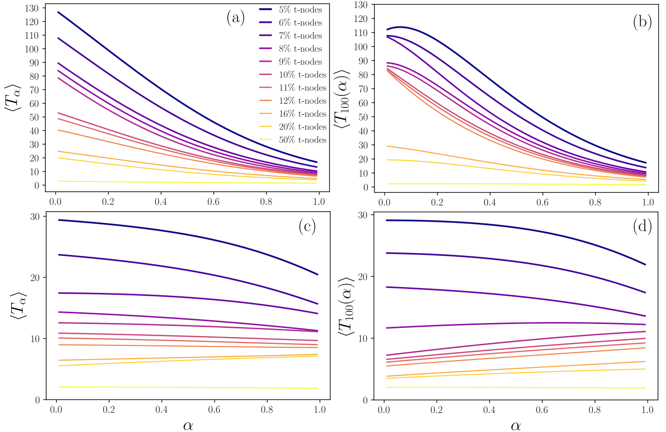
Figure 5: Global MFHT and MFHT as functions of the Sibuya index \alpha with uniform resetting probabilities to any node for some proportions of uniformly distributed t-nodes in the Watts-Strogatz and Barabási–Albert networks with size N = 500 . Frame (a) : \langle T_\alpha \rangle in Eq. (88) as a function of \alpha for the Watts-Strogatz network. Frame (b) : \langle T_{100}(\alpha) \rangle as a function of \alpha for the same network as in (a) with starting node i = 100 . Frames (c) and (d) present the same analysis for the Barabási–Albert network. The parameters of the considered graphs are identical as in Figs. 1 and 2. In all frames, we use the colors for the curves in panel (a) to code the proportion of t-nodes.
