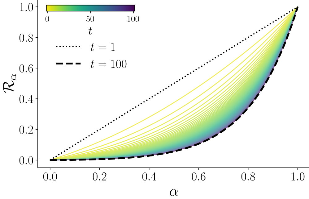
Figure 4: Sibuya resetting rate \mathcal{R}_\alpha of Eq. (84) as a function of \alpha and different values of t . The numerical results for 1 < t < 100 are coded with the colorbar, whereas the two extremal cases t = 1 and t = 100 discontinuous lines are depicted.
