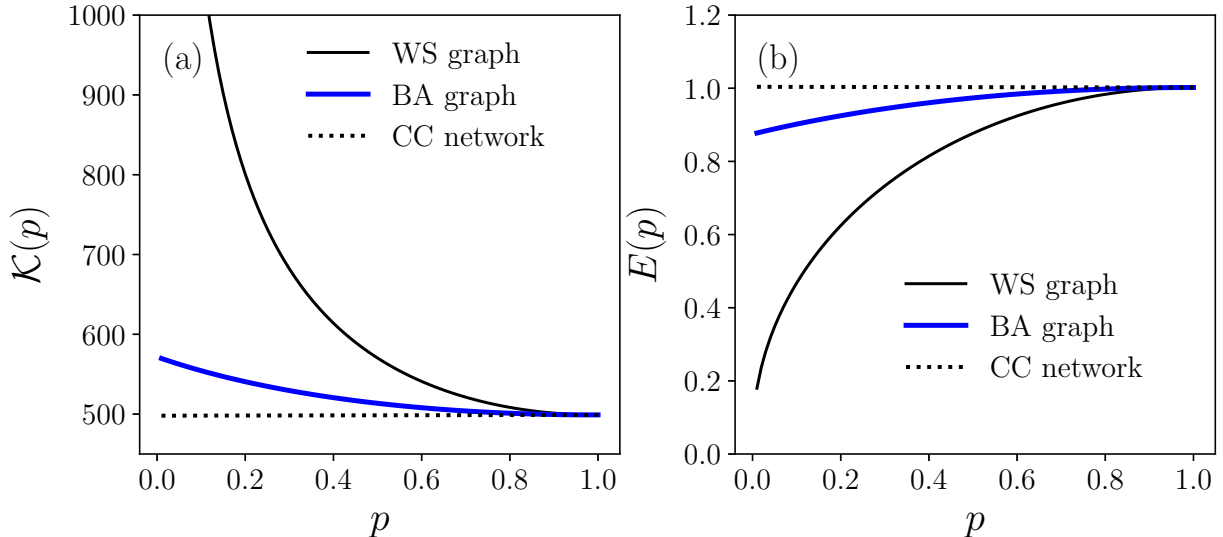
Figure 3: Comparison of the (a) Kemeny constant \mathcal{K}(p) and (b) search efficiency E(p) of Eq. (48) for the dynamics with resets in the Barabási-Albert and Watts-Strogatz graphs. The parameters are those of Figs. 1 and 2. The dotted lines denote the CC graph with \mathcal{K}_{CC} \approx N = 500 and E_{CC}(p) \approx 1 ( N \gg 1 ).
