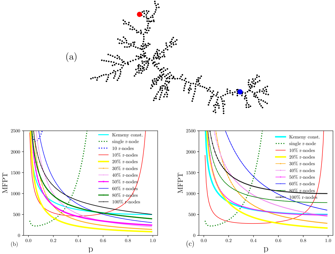
Figure 2: (a) Random search with resets between the starting node (blue) and the target node (red) in a Watts-Strogatz graph with N = 500 nodes, attachment parameter m = 2 (large-world) and rewiring probability 0.7. The Kemeny constant (Eq. (45)) is pictured in (b) and (c) in cyan color. We plot \langle T_{ij} \rangle (Eq. (43)) with respect to p for the starting node i = 100 and the target node j = 200 . (b) Same resetting scenarios and color codes as in Fig. 1(b) with uniform resetting probabilities ( R_r = R ) to the r-nodes. (c) Same resetting scenarios and color codes as in Fig. 1(c) with preferential resetting to the r-nodes ( R_r \propto K_r ).
