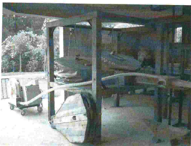
Figure 7: The ventilation system. For now the electric blower replaces the bellows.
