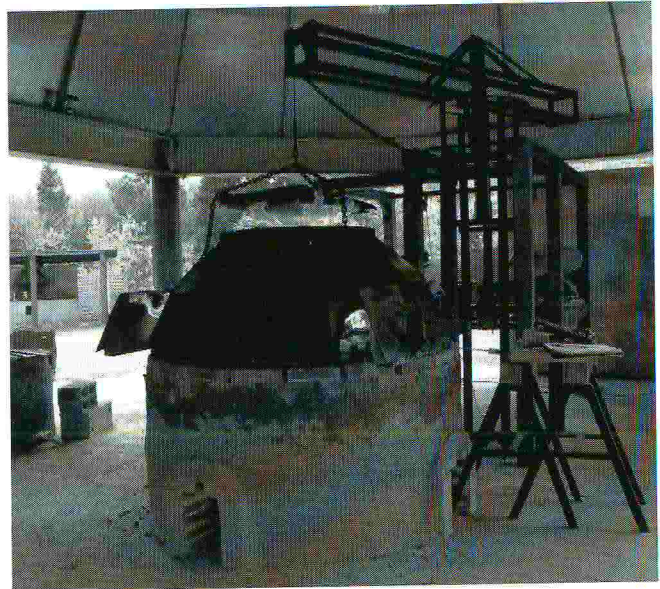
Figure 2: Experimental furnace during a firing.
