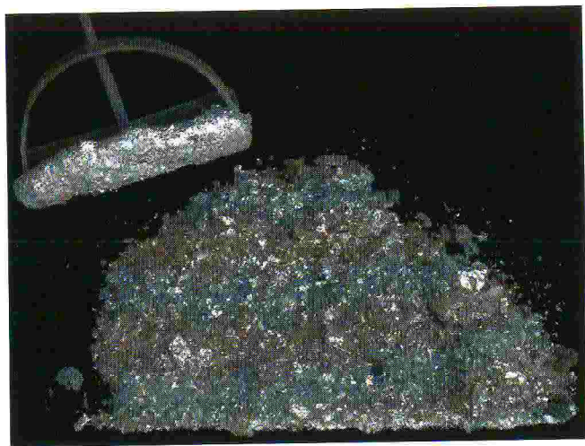
Figure 15: The experiments produced yellow crystalline flake litharge, some of which accumulated on the scraper.
