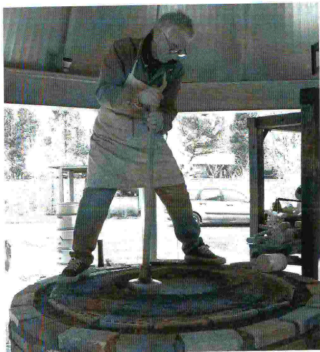
Figure 5: Experimental hearth making; the technique shown in Figure 4 is used.
