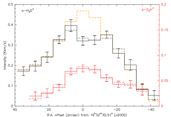
Fig. 5. Observed intensities along the horizontal cut (full lines with their error bar, corresponding to the spectra from Fig. 3) and corresponding model intensities (dashed lines). For ortho- \text{H}_2\text{D}^+ , we present an additional model (orange dashed line) for which the abundance is kept constant across the core. Para- \text{D}_2\text{H}^+ (in red) observations and model have their own intensity axis, also in red, on the right side of the plot.
