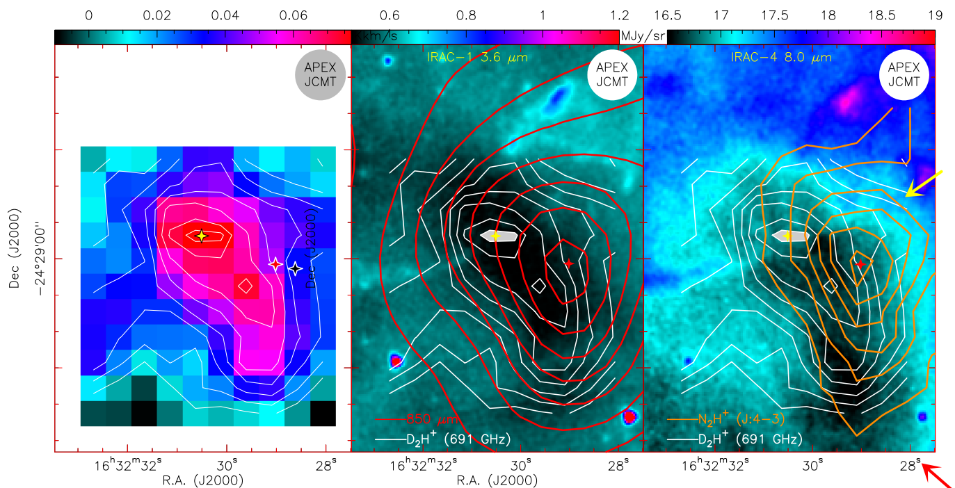
Fig. 1. Continuum and line emission images of IRAS 16293E. Left: Colour map of para- D_2H^+ integrated intensity emission with white contours (colour scale and white contours from 0.01 to 0.07 by 0.01 K km s^{-1} plus a contour at 0.075 K km s^{-1} = 1.5\sigma ) Centre: IRAC-1 image at 3.6 \mu m . White contours trace para- D_2H^+ as in the left panel. Red contours trace the SCUBA-II 850 \mu m emission ( 20 to 160 by 20 [ \approx 10\sigma ] MJy sr^{-1} ). Right: IRAC-4 image at 8.0 \mu m . White contours trace para- D_2H^+ as in the left panel. Orange contours trace the N_2H^+ ( J:4-3 ) integrated intensity ( 0.3 to 2.3 by 0.4 [ =12\sigma ] K km s^{-1} ). The yellow cross marks the centre of the D_2H^+ emission ( \alpha_{J2000}: 16^h 32^m 30.51^s , \delta_{J2000}: -24^\circ 28' 53.7'' , see also Fig. 2). The red cross marks the peak position of the dust and N_2H^+ ( J:4-3 ) emissions. The black cross (left panel) marks the position of the observation of D_2H^+ and H_2D^+ by Vastel et al. (2004). The yellow arrow traces the direction of the outflow from the IRAS16293-2422 protostellar system and the red arrow the outflow from WLY 2-69. The grey and white disks represent the JCMT and APEX beams after smoothing to 14'' .
