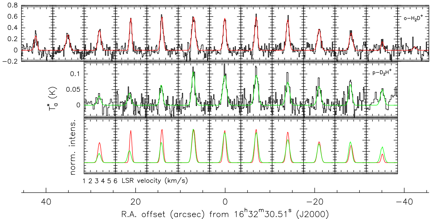
Fig. C.1. JCMT spectra of ortho-H 2 D + J_{KK'}:1_{10}-1_{11} (top row, velocity axis from 1 to 6 km s -1 ), and APEX spectra of para-D 2 H + J_{KK'}:1_{10}-1_{01} (middle row, velocity axis from 1 to 6 km s -1 ) across the cloud (the position of the cut is indicated in Fig. 2). Gaussian fits are overlaid in red and green, respectively. The same Gaussian fits with same colour code are reproduced in the bottom row, after normalization to the peak temperature for the +7'' spectrum, for a better comparison of the ratio variation and linewidth differences between the two isotopologues.
