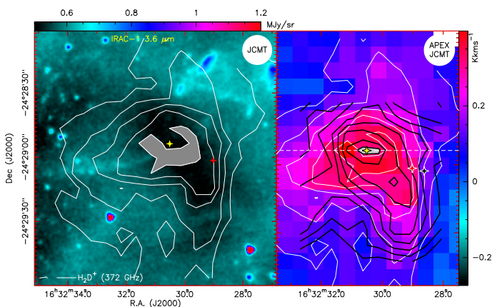
Fig. 2. Left: IRAC-1 image at 3.6 \mu m . White contours trace ortho- H_2D^+ . The filled grey contour marks the strongest emission (contours from 0.10 to 0.34 by 0.06 [ =2.6\sigma ] K km s^{-1} ). Right: para- D_2H^+ and ortho- H_2D^+ maps. Same map of para- D_2H^+ (black contours) as in Fig. 1 superimposed on the ortho- H_2D^+ map (colour scale, plus white contours as in left panel). The yellow, black, and red crosses are as in Fig. 1. D_2H^+ , H_2D^+ , and N_2H^+ spectra along the cut traced by the dashed line are displayed in Fig. 3
