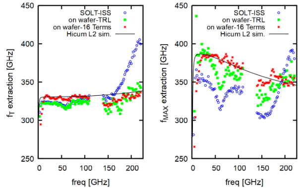
FIGURE 9. Determination of a) f_T (defined as H_{21} \times \text{freq} ), b) f_{MAX} (defined as U^{1/2} \times \text{freq} ) versus frequency of the transistor ( A_E=0.09 \times 5 \mu\text{m}^2 ) at V_{BE}=0.9 V and V_{CB}=0 V.
