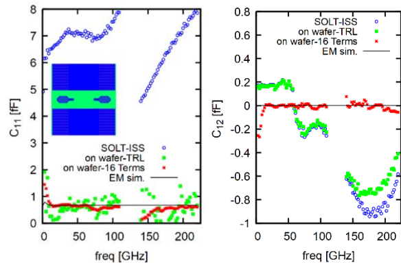
FIGURE 5. a) C 11 and b) C 12 capacitance of the pad-open structure versus frequency; Comparison of the different calibration method (SOLT-ISS, on wafer TRL, on wafer 16 terms, EM simulation).
