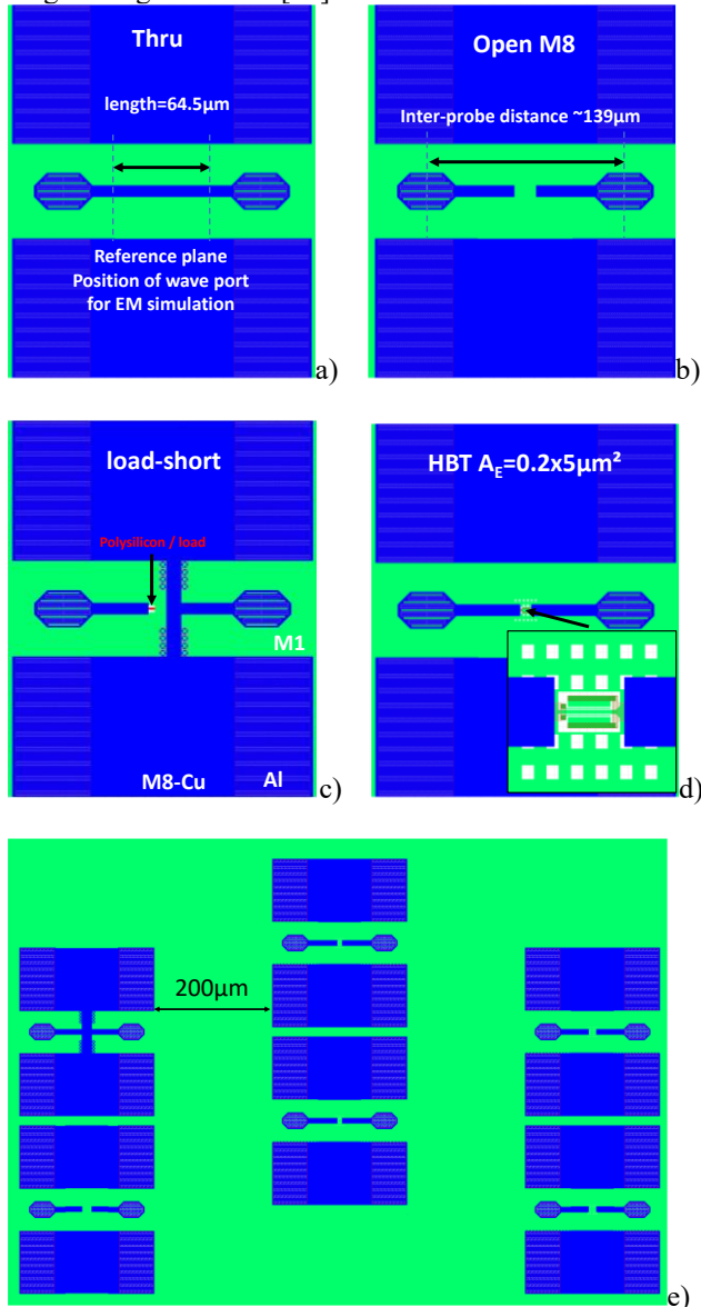
FIGURE 1. Layout of the principal test-structures highlighting distance between probes (dummies have been simplified for clarity); a) Thru, b) Open-M8, c) the load-short structure is also illustrative for the load-load or short-short structure using the symmetry, d) HBT, e) floorplan view of some of the structures highlighting the arrangement.
