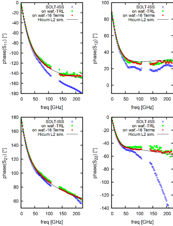
FIGURE 8. Measurement of phase of S parameters versus frequency of the transistor ( A_E=0.09 \times 5 \mu\text{m}^2 ) at V_{BE}=0.9 V and V_{CB}=0 V.
