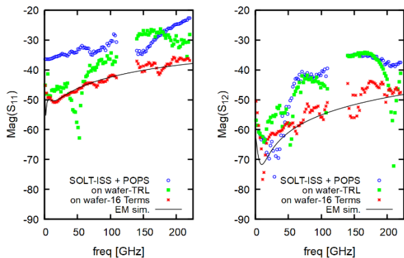
FIGURE 4. a) Magnitude of S 11 and b) of S 12 of the load-load structure versus frequency; Comparison of the different calibration method (SOLT-ISS, on wafer TRL, on wafer 16 terms, EM simulation). (6 calibration standards used for 16-terms method)
