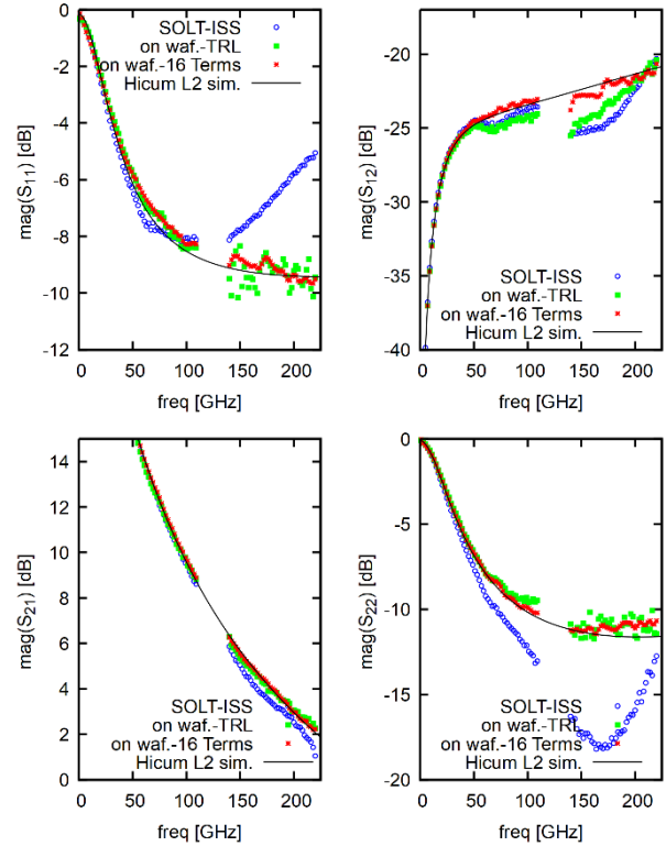
FIGURE 7. Measurement of magnitude of S parameters versus frequency of the transistor ( A_E=0.09*5\mu m^2 ) at V_{BE}=0.9V and V_{CB}=0V .
