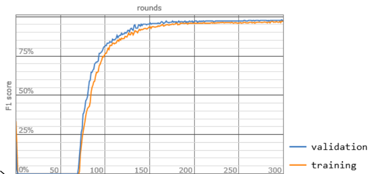
MatthewsCorrelationCoefficient ->
