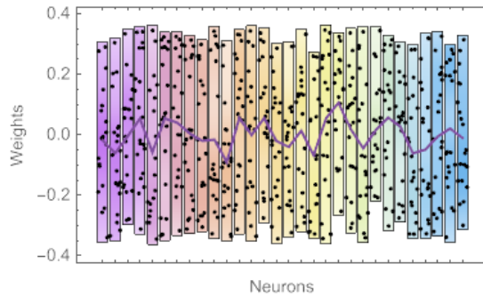
Weight Distributions using Xavier initialized Weights of the 30 Neurons
