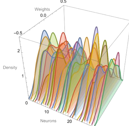
Weight Distributions using Xavier initialized Weights of the 30 Neurons
