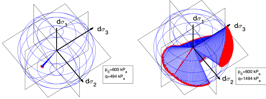
Figure 4: Some cones of unstable loading directions obtained with the Darve's model calibrated on a dense sand. Prunier et al. (2009c,b,a). The first one is reduced to single direction and corresponds to a stress state on the bifurcation limit. The second one corresponds to a stress state within the bifurcation domain and strictly inside the plasticity limit.
