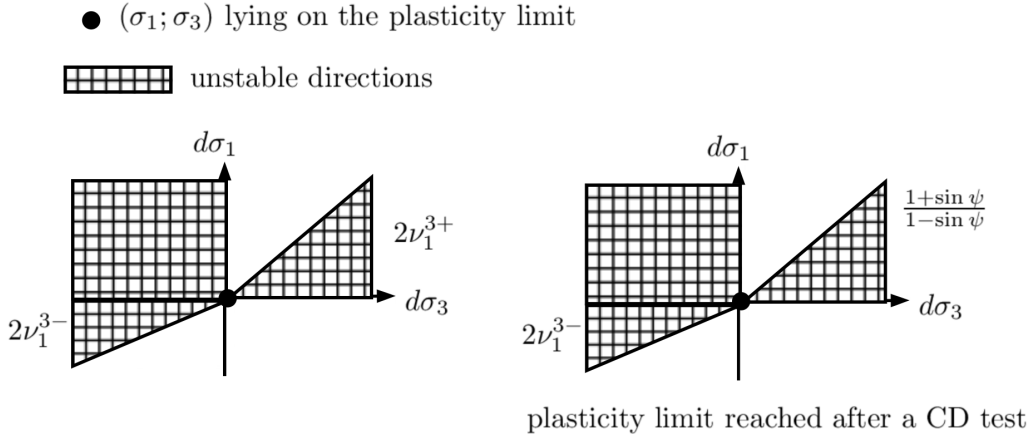
Figure 7: instability secant planes (degenerated cones with an infinite wider axis) for a stress state lying on the plasticity limit. Sum up of equations 66 to 77. 0 , 2\nu_1^{3\pm} and \frac{1+\sin \psi}{1-\sin \psi} are the slope of the instability secants planes.
