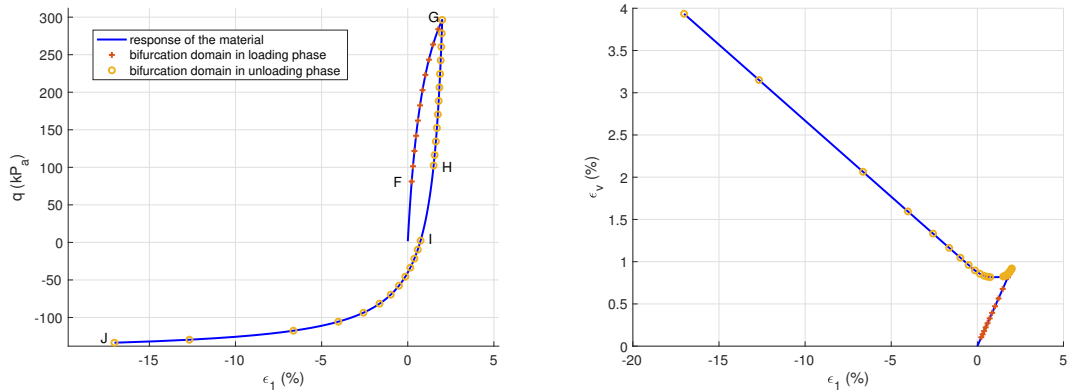
Figure 16: Response of the Octolinear model calibrated on a loose Hostun sand to an alternated drained triaxial path
