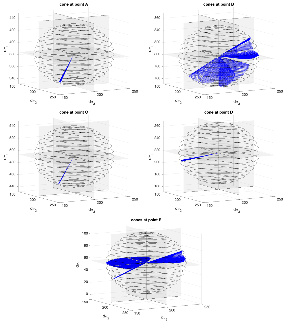
Figure 12: Development of instability cones along the stress path for the dense sand.
