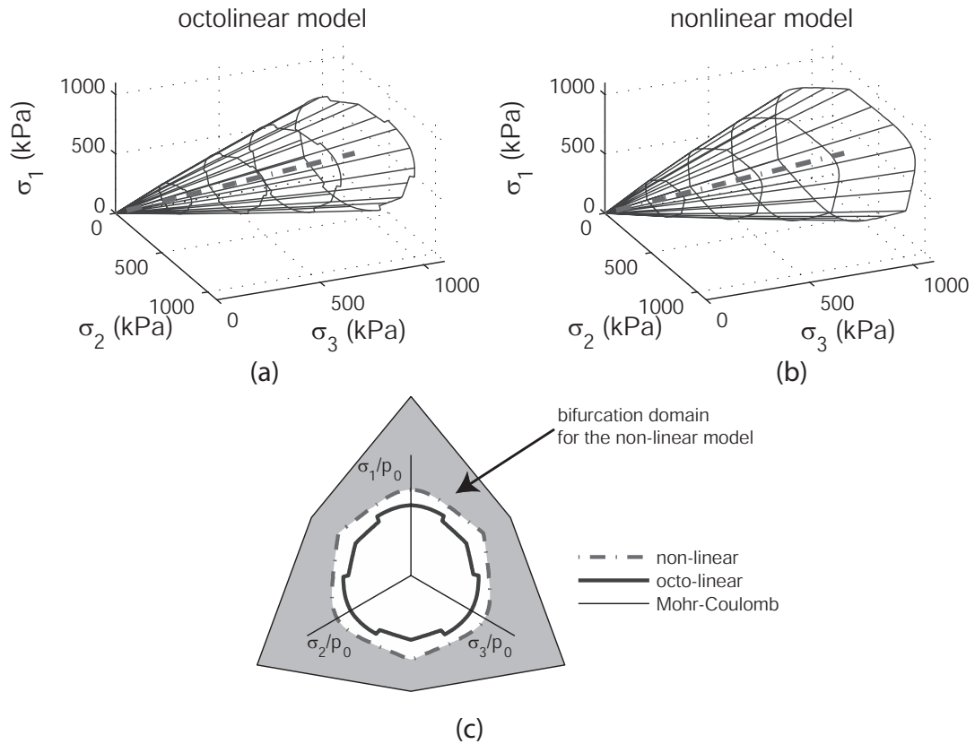
Figure 3: Bifurcation limit for the elasto-plastic models of Darve Darve et al. (1995) calibrated on a dense sand. Prunier et al. (2009c,b,a)
