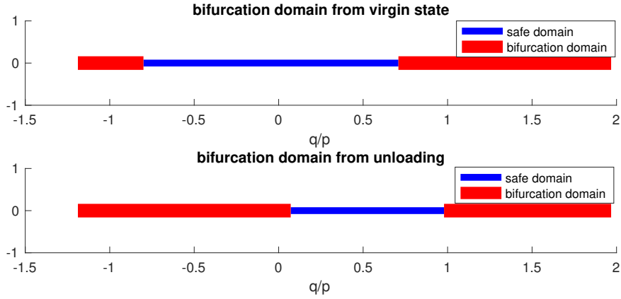
Figure 11: Evolution of the bifurcation domain for a dense sand. At the top, the bifurcation domain obtained starting from the initial isotropic state. At the bottom, the one obtained during the unloading.
