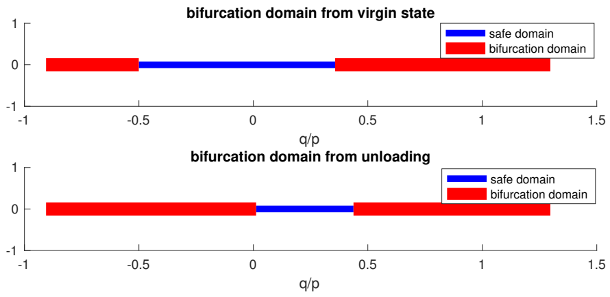
Figure 17: Evolution of the bifurcation domain for a loose sand. At the top, the bifurcation domain obtained starting from the initial isotropic state. At the bottom, the one obtained during the unloading.
