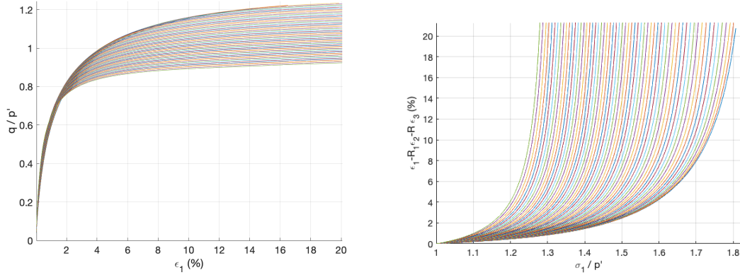
Figure 6: response of the octo-linear model calibrated on a loose Hostun sand to radial loading paths in the deviatoric plane
