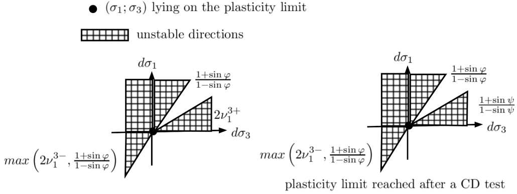
Figure 8: instability secant planes (degenerated cones with an infinite wider axis) for a stress state lying on the plasticity limit. Sum up of equations 66 to 77 and merging the plasticity limit condition. 0 , 2\nu_1^{3\pm} and \frac{1+\sin \psi}{1-\sin \psi} are the slope of the instability secants planes. \frac{1+\sin \varphi}{1-\sin \varphi} is the slope of the Mohr-Coulomb plane.
