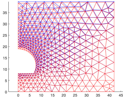
Figure 13: Initial mesh at the beginning of the excavation phase in blue, and deformed mesh ( \times 10 ) at the end of the excavation phase in red
