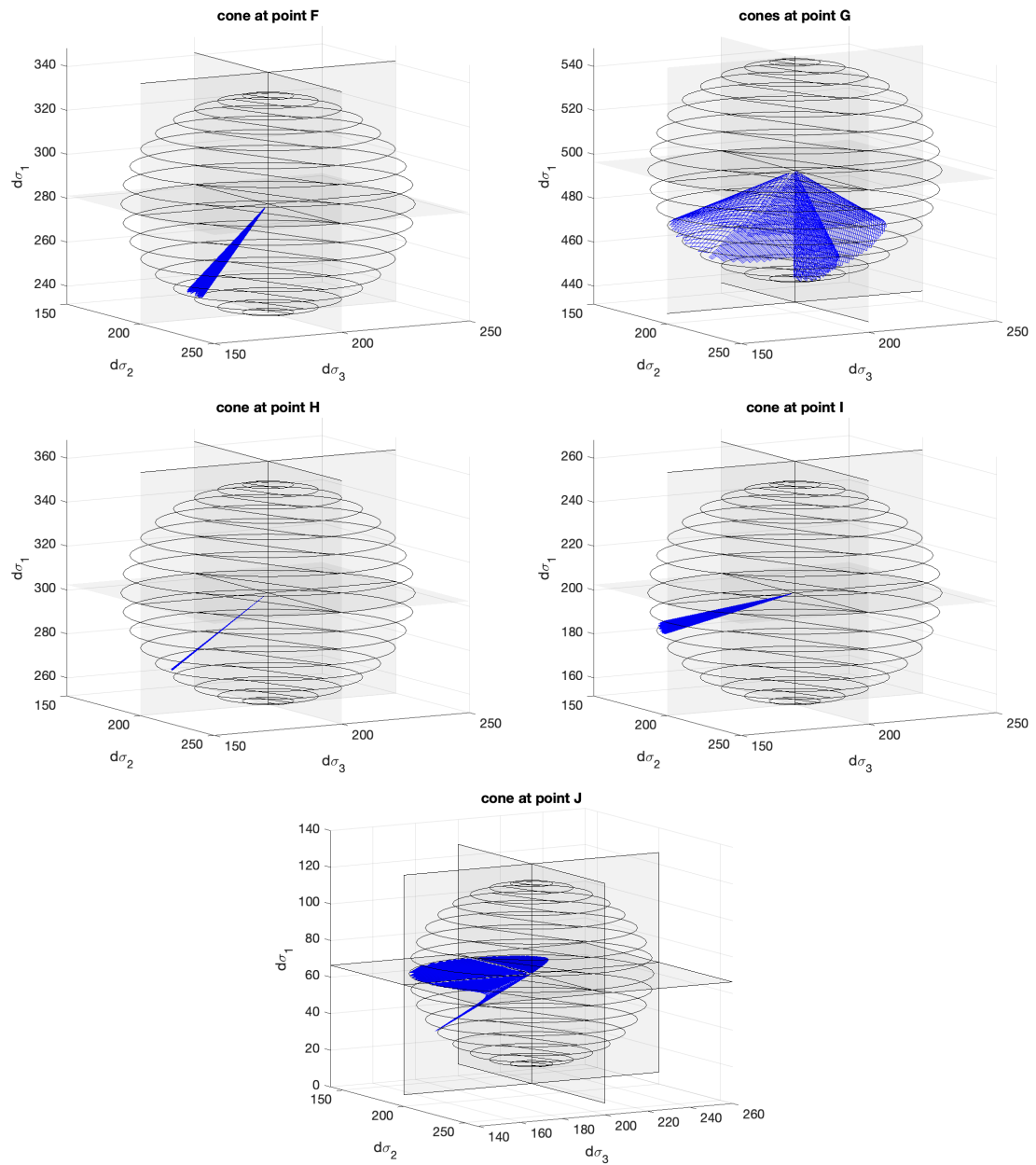
Figure 18: Development of instability cones along the stress path for the loose sand.
