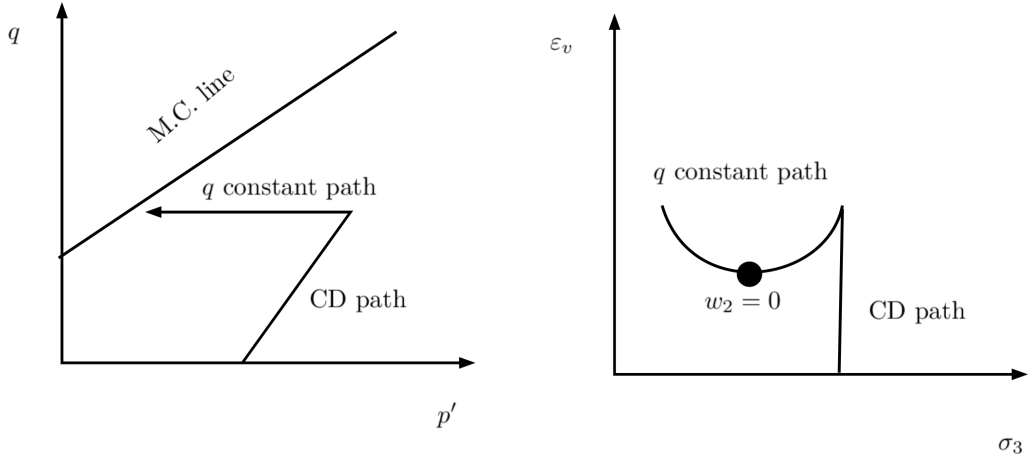
Figure 5: Sketch of the unloading path at q = cst and typical response of some geomaterials to this path.
