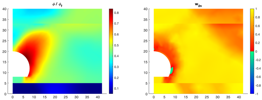
Figure 14: Mobilized friction angle divided by the friction angle at failure (left). Local normalized second order work (right).
