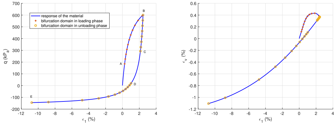
Figure 10: Response of the Octolinear model calibrated on a dense Hostun sand to an alternated drained triaxial path
