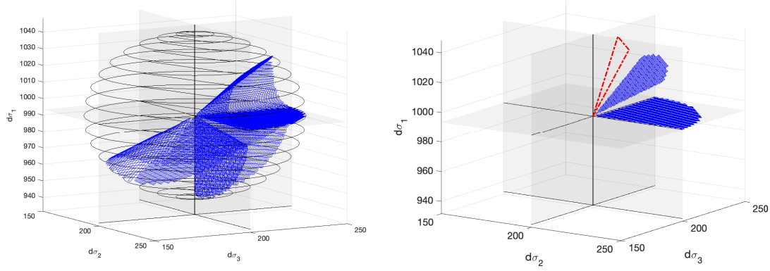
Figure 9: 3D instability cone get with the octolinear model of Darve for a stress point in the vicinity of the Mohr-Coulomb envelop. On the right figure we only kept the cone for the tensorial zone ( d\sigma_1 > 0, d\sigma_2 > 0, d\sigma_3 > 0 ) and added the tangent plane to the Mohr-Coulomb envelop in dashed line.
