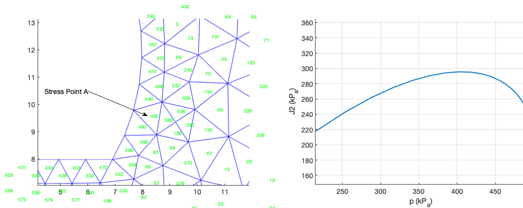
Figure 15: Loading path of point A during the excavation phase.
