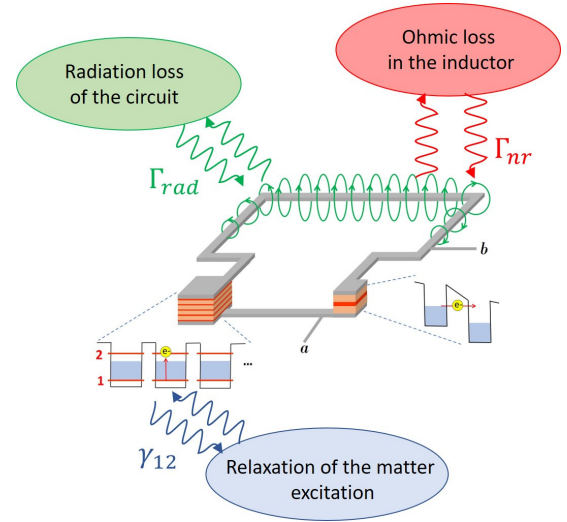
FIG. 6. Schematics indicating the various dissipation mechanisms for the system together with the definitions of the corresponding coupling rates.
