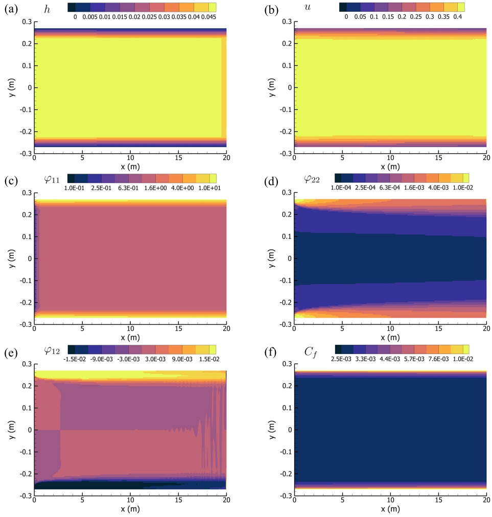
Figure 17: Numerical simulation of the experiment 23 of Yuen (1989): (a) depth h (m); (b) average velocity U (m/s); (c) entrophy component \varphi_{11} ( s^{-2} ); (d) entrophy component \varphi_{22} ( s^{-2} ); (e) entrophy component \varphi_{12} ( s^{-2} ); (f) Friction coefficient C_f .
