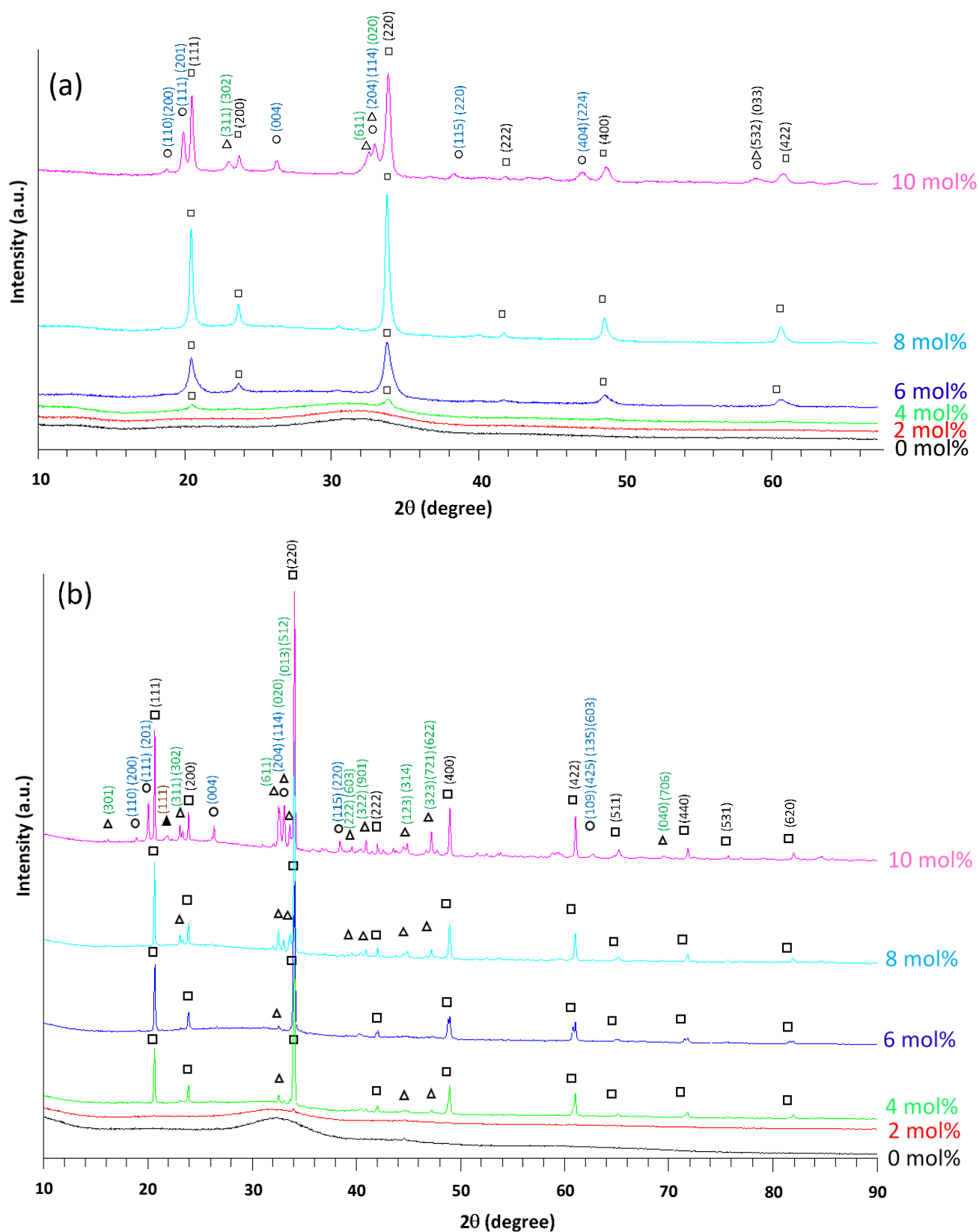
Figure 2. XRD patterns recorded at room temperature of the quenched (a) and slowly cooled (b) samples increasing P_2O_5 contents (0-10 mol%). □ ( \gamma - Na_3PO_4 PDF#:00-031-1318), ○ ( Na_4P_2O_7 PDF#:04-018-4331), △ ( NaCaPO_4 PDF#:04-0016-6900), ▲ ( SiO_2 cristobalite PDF#:04-013-9484).
