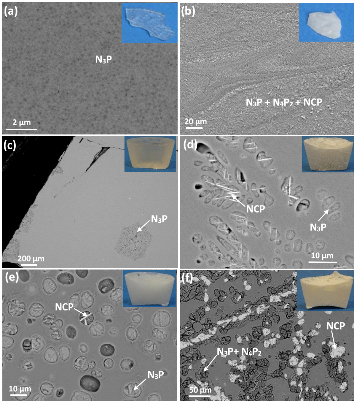
Figure 1. SEM images (backscattered electrons) of quenched samples with 8% (a) and 10% (b) P_2O_5 and slowly cooled samples with 2% (c), 4% (d), 6% (e) and 10% P_2O_5 . N_3P ( \gamma-Na_3PO_4 ), NCP ( NaCaPO_4 ), N_4P_2 ( Na_4P_2O_7 ). Macroscopic pictures of the samples are shown in inset.
