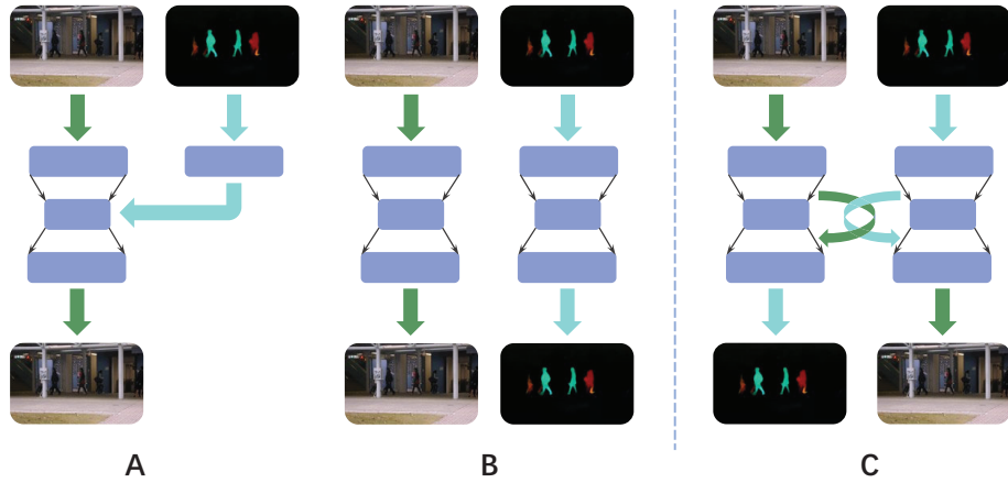
Figure 1: Comparison of methods: A uses optical flow features as a supplement to video frame appearance features to improve prediction accuracy; B uses parallel prediction of appearance features and optical flow features to build a joint prediction loss error; C is the proposed strong consistency collaborative training framework.
