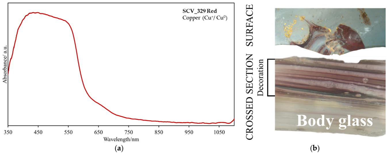
Figure 16. (a) UV-Vis absorption spectrum of red glass layer performed on SCV_329 fragment, revealing the discernible influence of monovalent (Cu + ) and metallic (Cu 0 ) copper. (b) Close-up of the SCV_245 fragment under the surface and cross-section.
