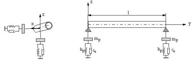
Figure 5: Rotor model
