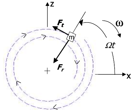
Figure 12: backward precession
