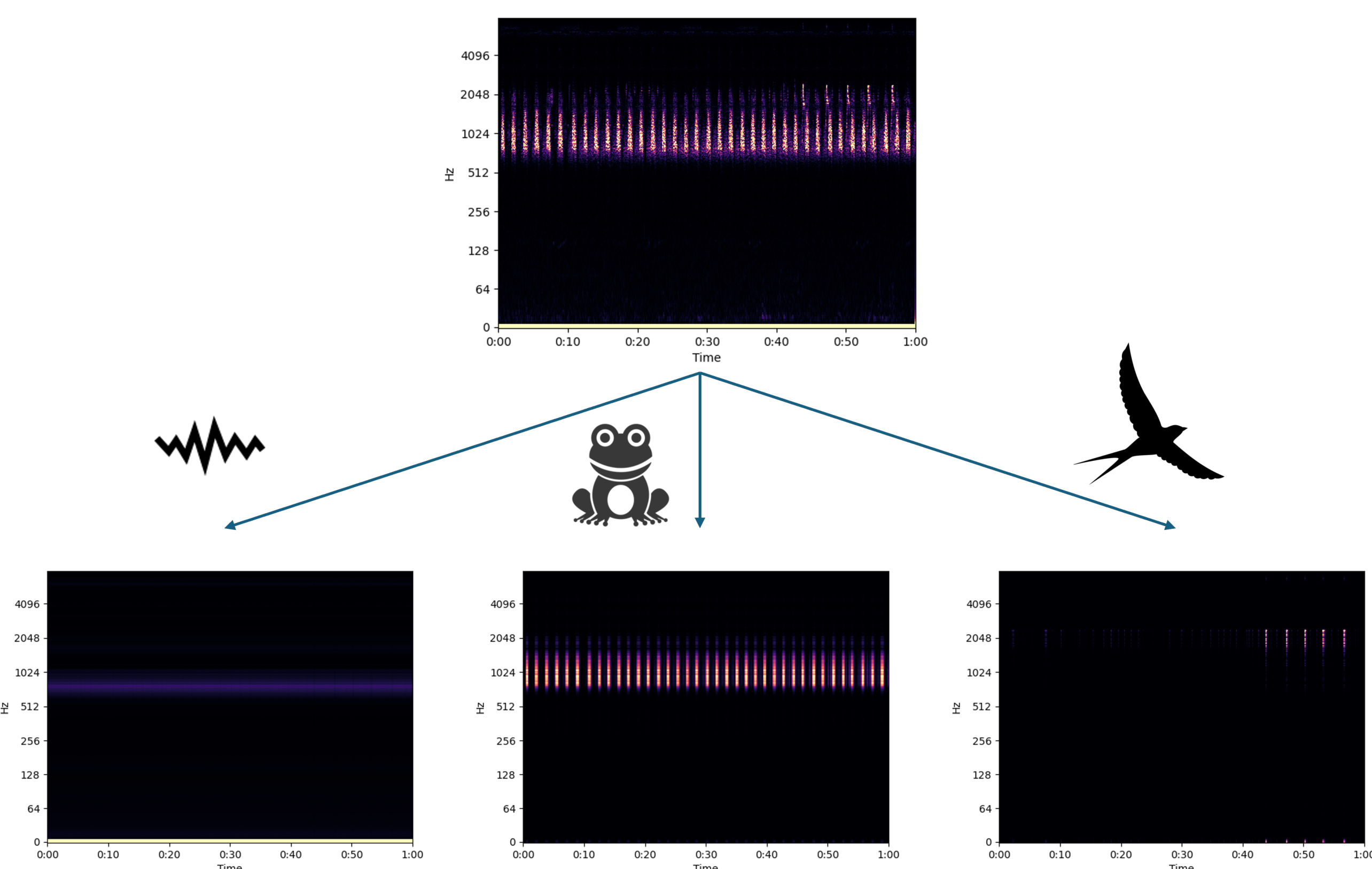
Figure 2. Source separation with NMF.
