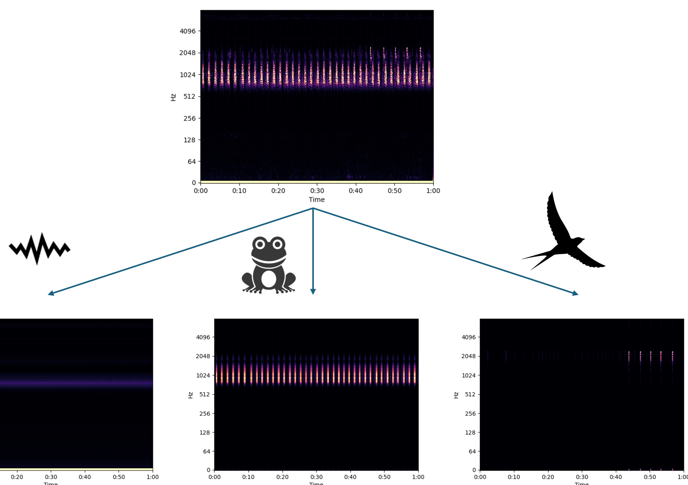
Figure 2. Source separation with NMF.
