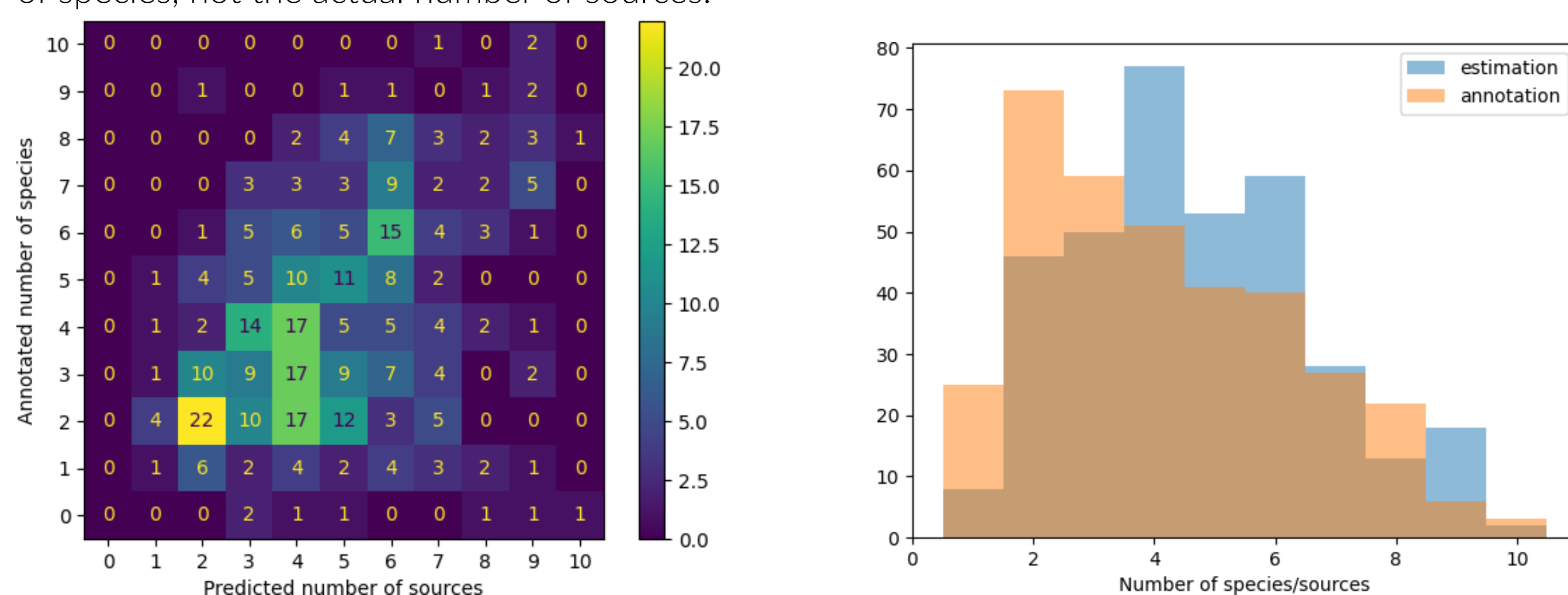
(a) Confusion matrix of NMF-estimated number of sources versus annotations of species.
