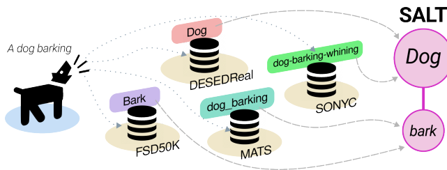
Figure 1: Illustration of SALT’s standardization process. Dataset labels are systematically mapped to a standard label that ensures cross-dataset compatibility.
