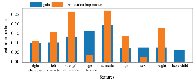
Fig. 6: Feature importance: Our XGBoost model could make human like distribution decisions with an accuracy of 87.2%. To understand which features are important to predict the human decisions, we looked at the ‘gain’ (blue) and ‘permutation importance’ (orange) of various features. The first four features are those for the characters to whom a participant distributes items in each ‘scenario’ (5th feature in the figure) of reward, effort or risk. The last four features are features of the decision making participant. We found the perceived strength difference and age difference of the characters, as well as the age and height of a participant to be the most importance features to predict human decision behaviors.
