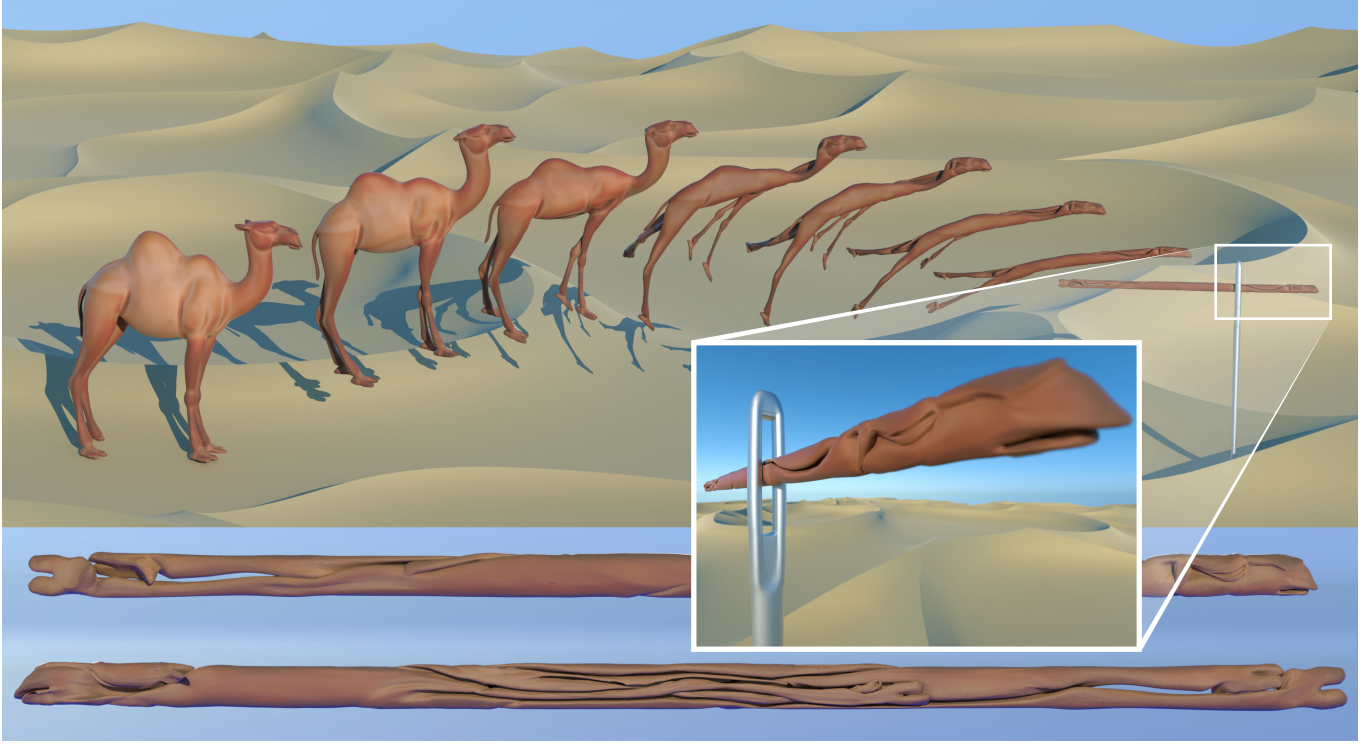
Fig. 14. Passing a camel through the eye of a needle. The initial mesh ( far left ) is first progressively compressed into a cylinder ( far right ); we then find a geodesic between initial and compressed states ( left to right ). Bottom : close-up of compressed geometry from left/right sides; inset shows occluded piece.
