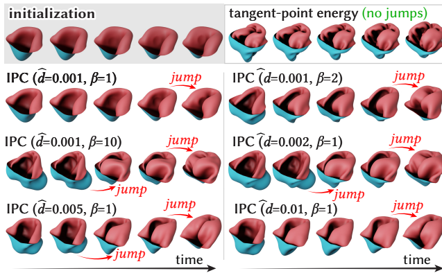
Fig. 20. When using the IPC barrier as potential energy in our framework, we struggle to find geodesics without sudden “jumps” (more obvious in supplementary video), even with good initialization (top left). Here using the IPC barrier energy for repulsion fails to yield a smooth surface eversion, even after extensive parameter tuning (bottom three rows). A TPE-based formulation easily finds smooth trajectories without jumps (top right).
