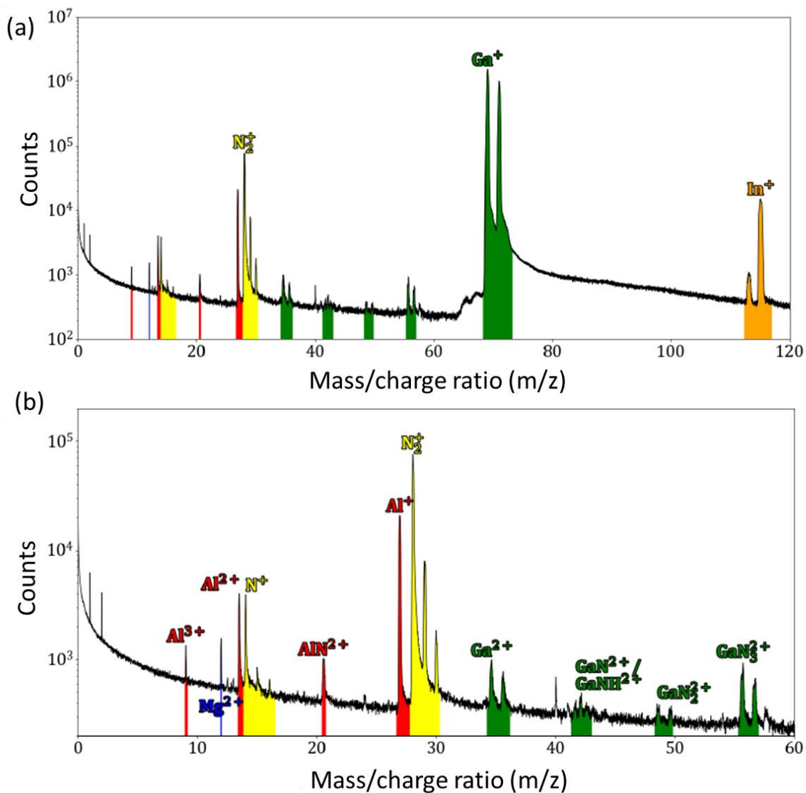
Figure S1. APT Mass/Charge spectrum of one LD-TJ sample. (a) Global spectrum and (b) zoom into the mass spectrum showing the species with a mass-to-charge ratio below 60 amu. The mass windows which are used for the atom identification of the APT reconstruction are color coded: green intervals correspond to Ga-containing species, red intervals to Al-containing species, orange to In-containing species, yellow to molecular or atomic Nitrogen, blue to Magnesium.
