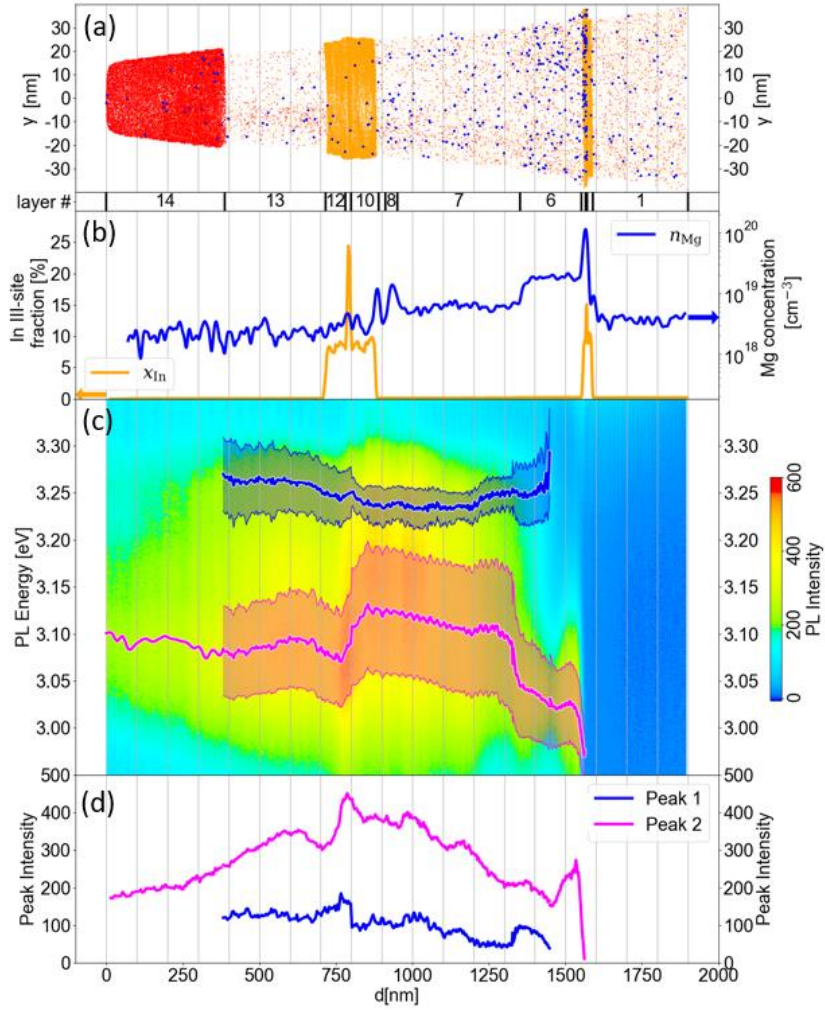
Fig. 3. Correlated PAP data as a function of the reconstructed depth coordinate d . (a) 5 nm thick slice of the reconstructed volume, displaying Al (red), In (orange) and Mg (blue) atom positions. Notice that the spatial coordinate x scale is expanded for clarity and the layer number is reported at the bottom of the graph (b) Composition profiles displaying the In III-site fraction (orange, left-hand ordinates) and the Mg concentration (blue curve, right-hand ordinates) (c) Sequence of PL spectra. The peak energies E_{PL,m}(i_{PL}) of sub-bandgap peaks 1 (pink) and 2 (blue), along with the width of the spectral component \sigma_{m,i_{PL}} have been superimposed to the color plot. (d) Evolution of the intensities I_m(i_{PL}) of peak 1 (pink) and 2 (blue). An animated version of parts (a) and (c) is available as Supplemental Material [36].
