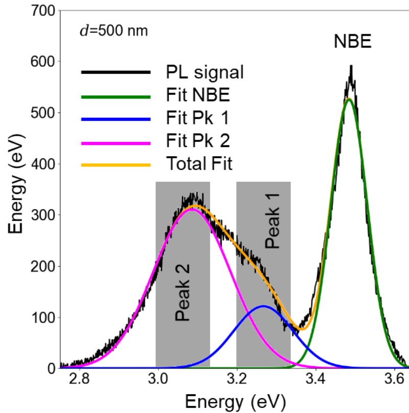
Fig. 4. PL spectrum indexed by i_{PL}=75 , corresponding to the depth coordinate of the reconstructed volume d=500 nm (layer 13). The graph also traces the gaussian functions used for the fit, along with the spectral interval in which the investigated contributions of peak 1 (3.19-3.3 eV) and peak 2 (2.98-3.17 eV) are located.
