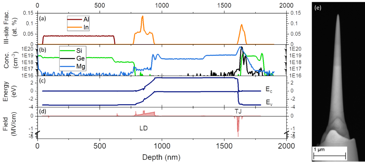
Figure 1. (a) SIMS profile of the III-site fraction of Al and In, (b) SIMS profile of the concentration of Si (green), Ge (black) and Mg (blue) doping. (c) Band diagram simulated based on the nominal layer thicknesses, III-site fractions and doping concentrations, (d) corresponding field distribution along the
