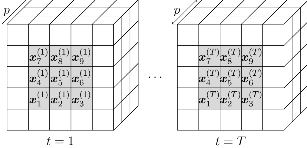
Figure 1: Illustration data notation for change detection test in a MITS.
