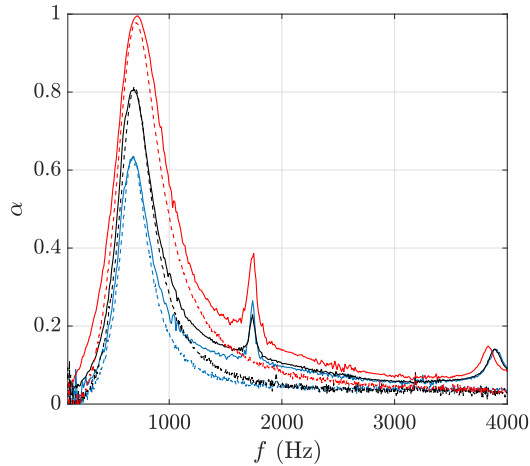
Figure 2: Comparison of experimental (solid line) and numerical (dashed line) absorption coefficient \alpha for several incident SPL: — 77 dB, — 117 dB and — 127 dB
