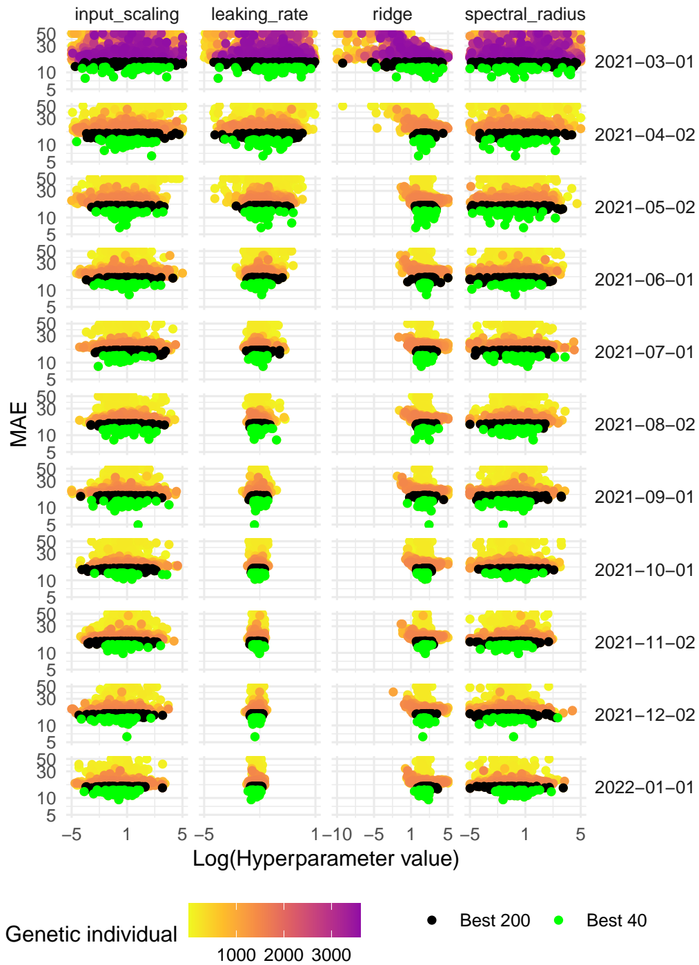
Figure 9. RC-GA with 20 reservoirs for hyperparameter optimization.
