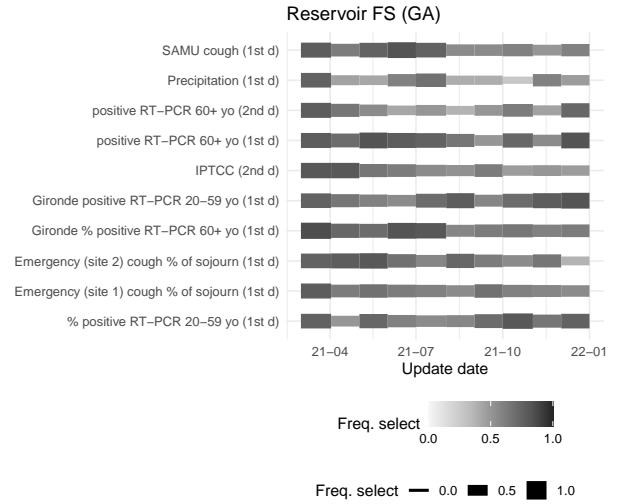
Figure 3. Feature selection by GA among the 40 best hyperparameter sets at each hyperparameter update. Only 10 most selected features at 2021-03-29 are shown.
