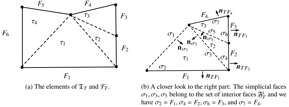
Figure 1: An illustration of the sets \mathfrak{T}_T, \mathfrak{F}_T and \mathfrak{F}_T^i for a given element T \in \mathcal{T}_h in \mathbb{R}^2 .
